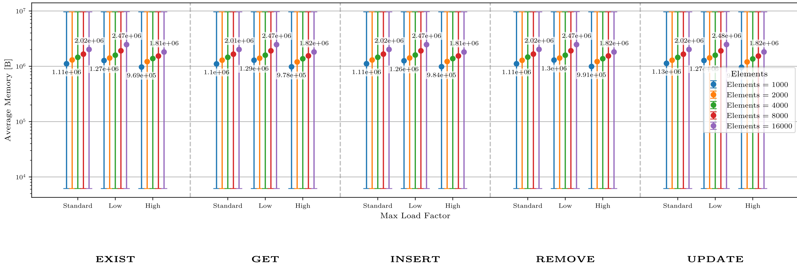
Memory by Operation and Max Load Factor
