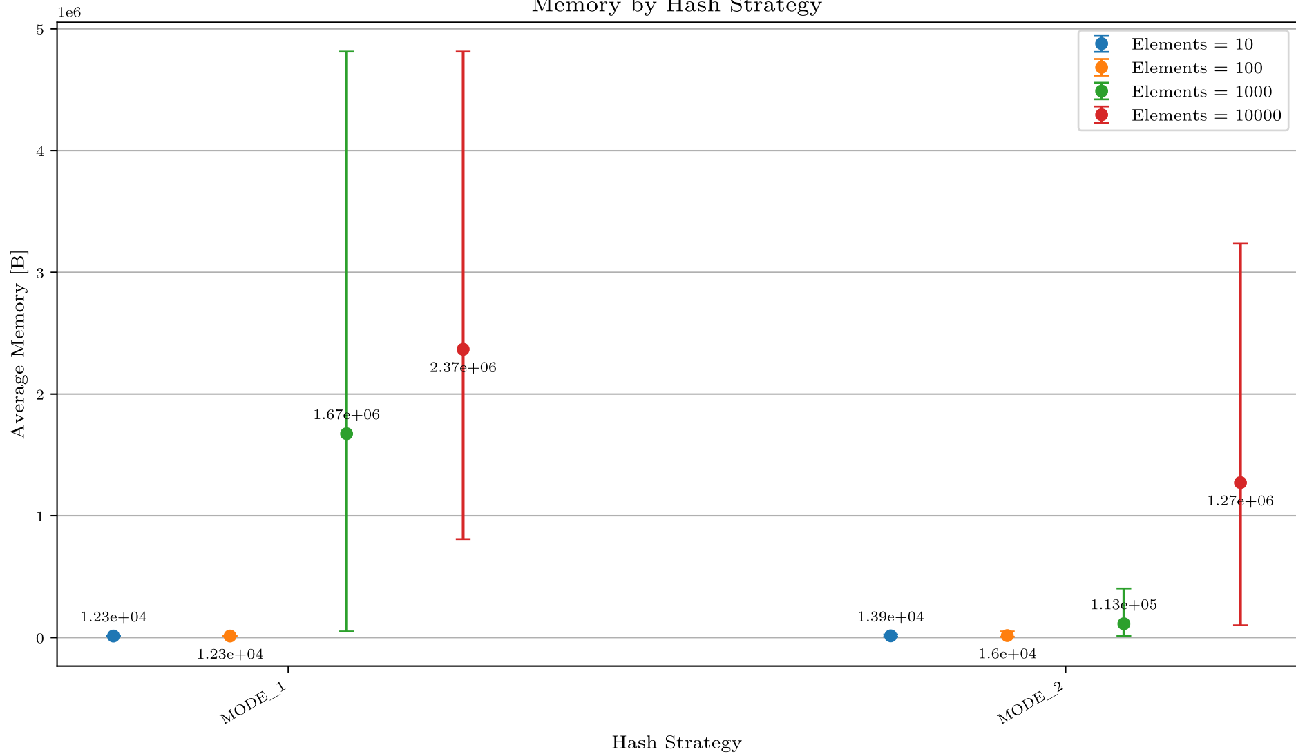
Memory by Hash Strategy
