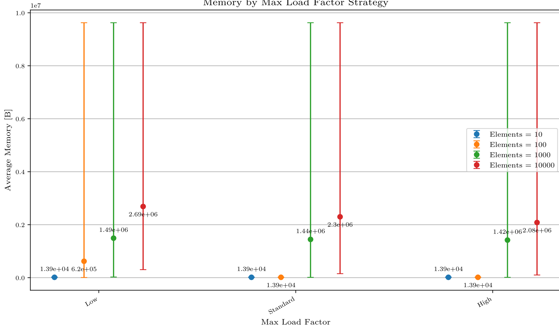
Memory by Max Load Factor Strategy
