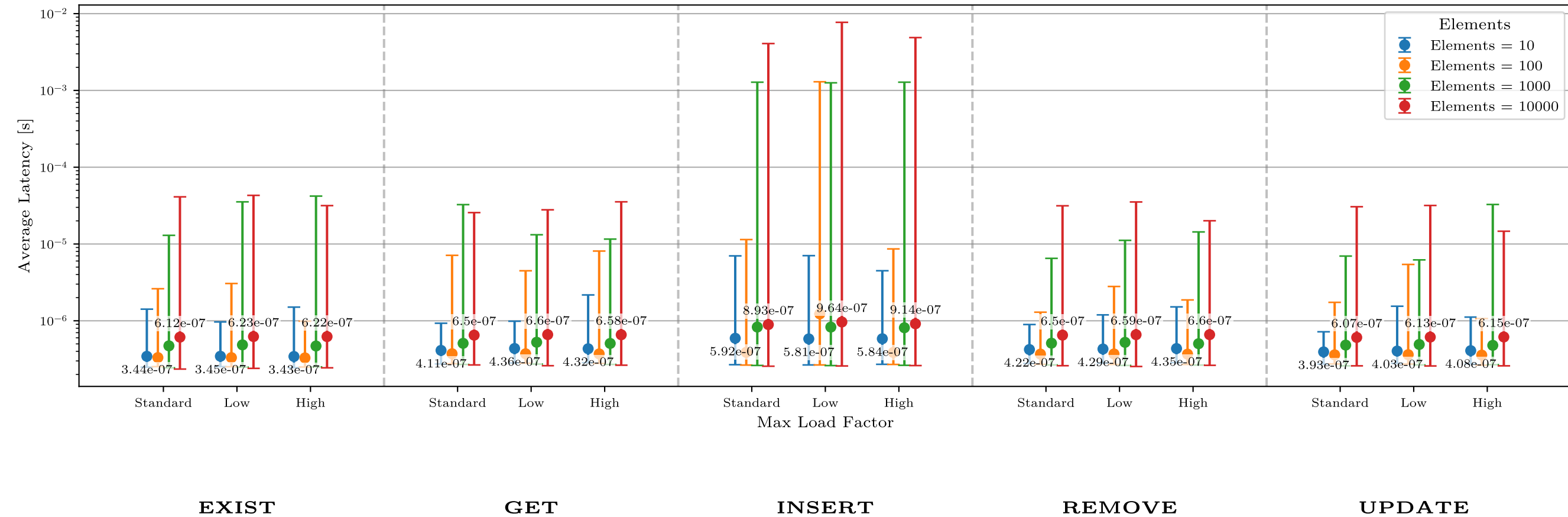
Latency by Operation and Max Load Factor
