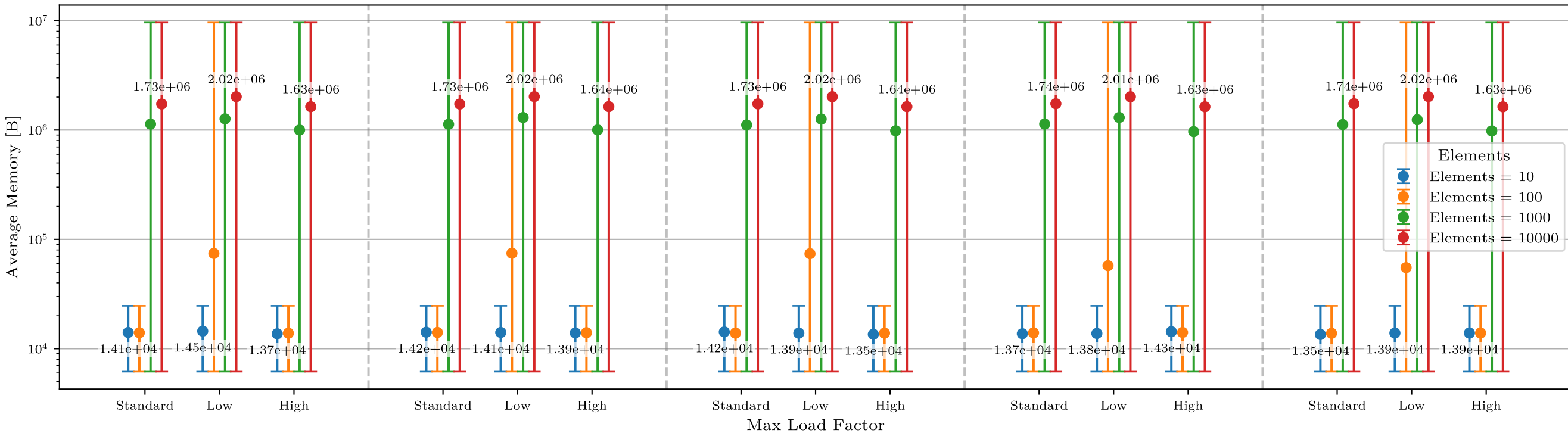
Memory by Operation and Max Load Factor
