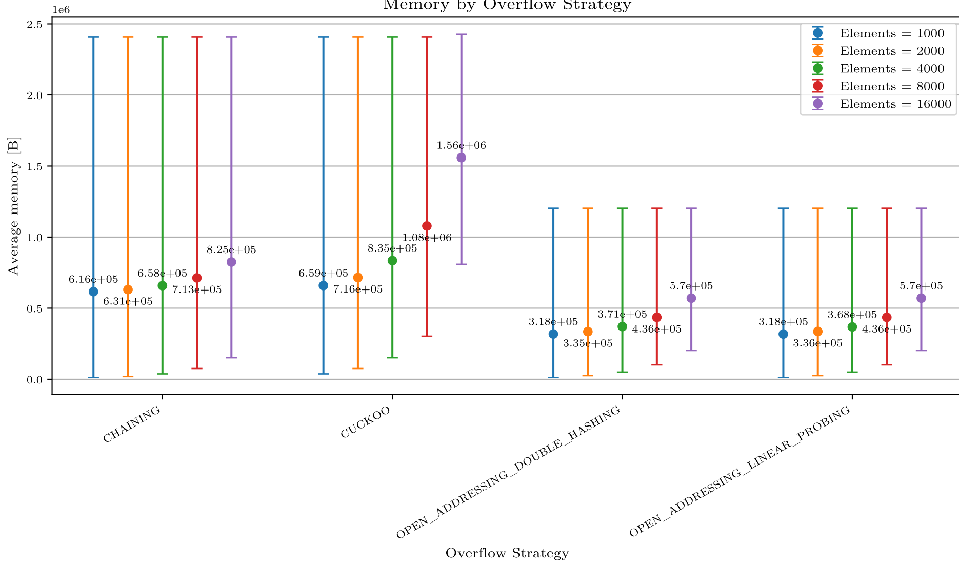
Memory by Overflow Strategy
