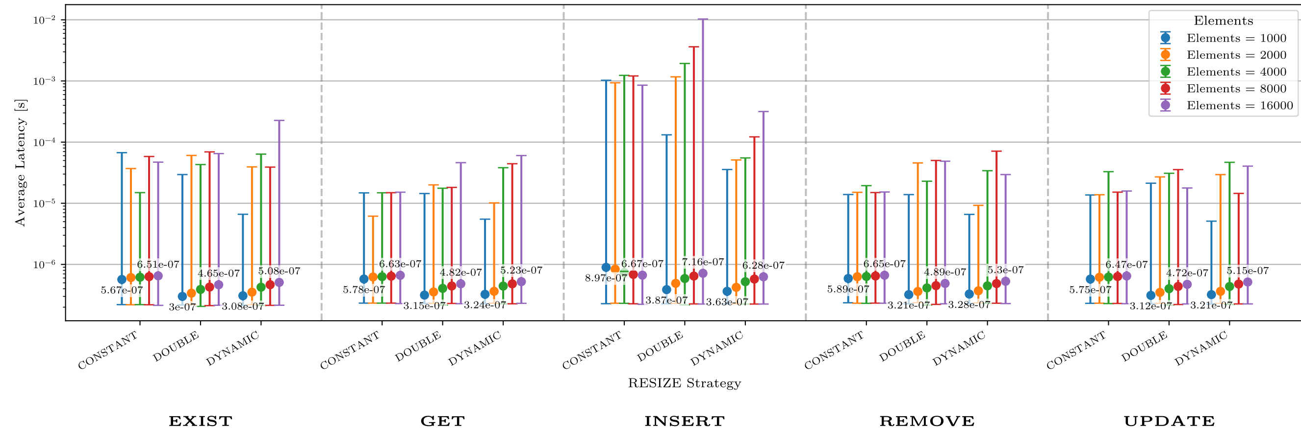
Latency by Operation and Resize Strategy
