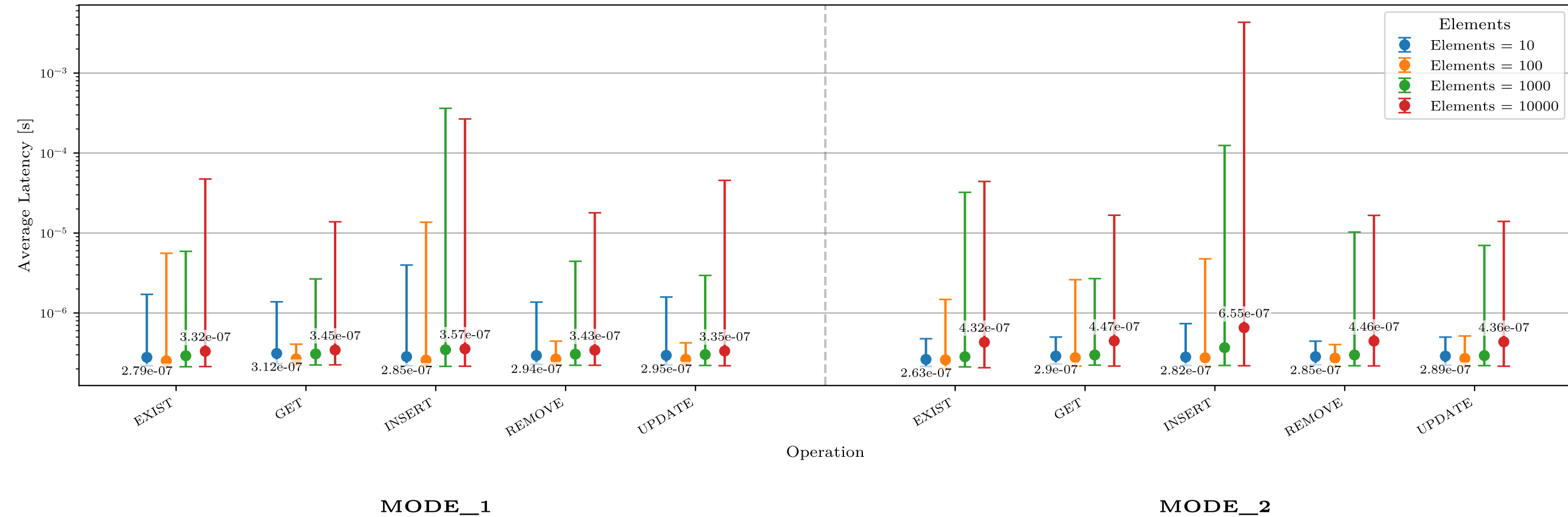
Latency by Operation and Hash Strategy
