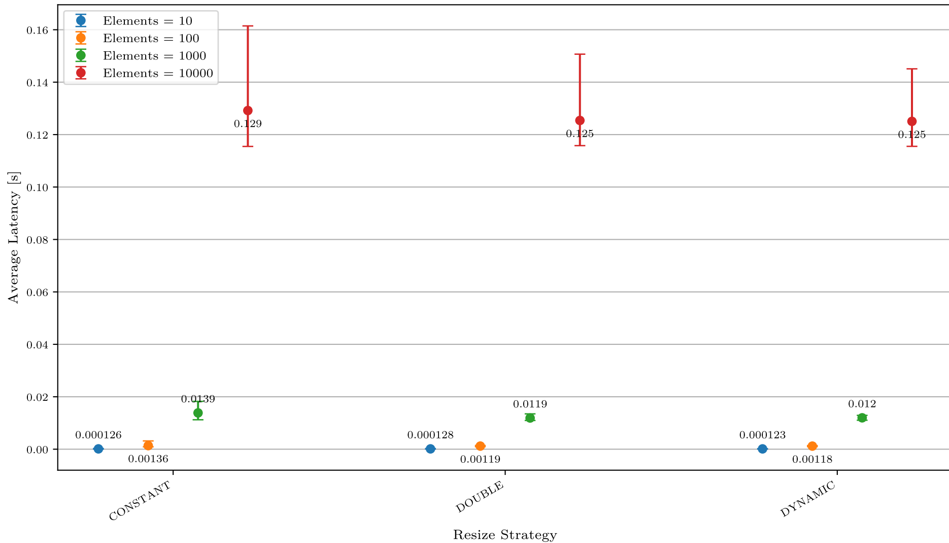
Latency by Resize Strategy
