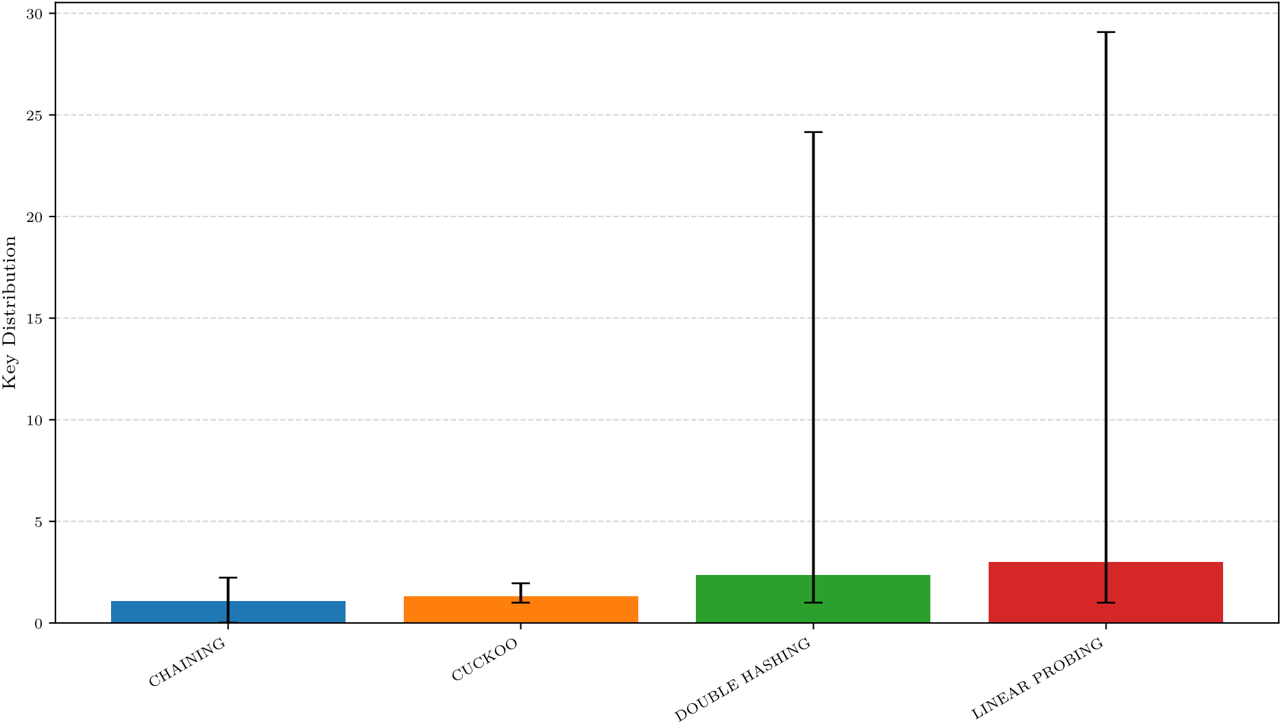
Key Distribution by Overflow Method (Elements = 10000)
