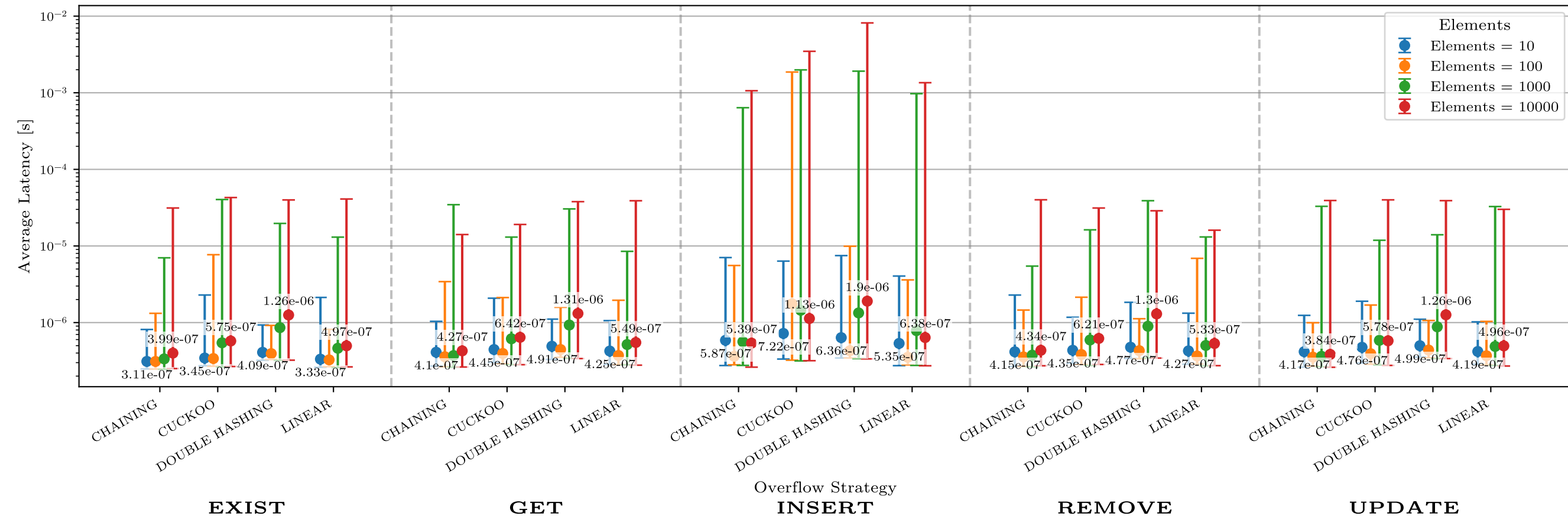
Latency by Operation and Overflow Strategy
