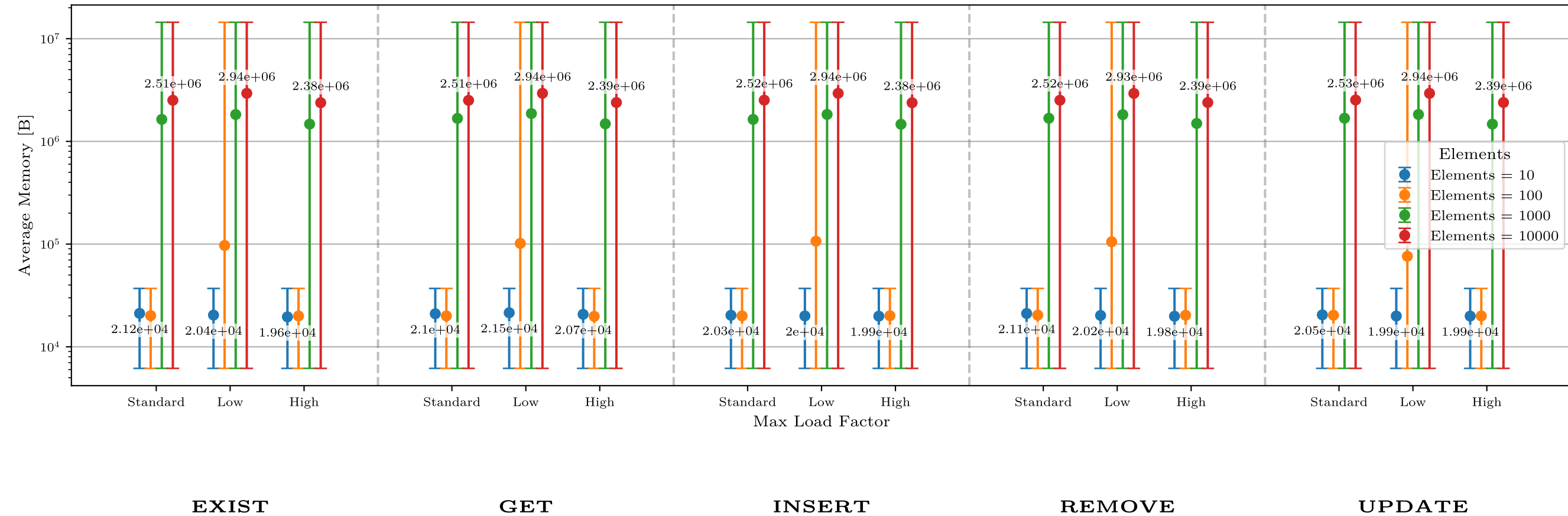
Memory by Operation and Max Load Factor
