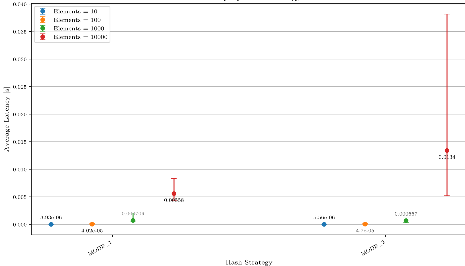
Latency by Hash Strategy
