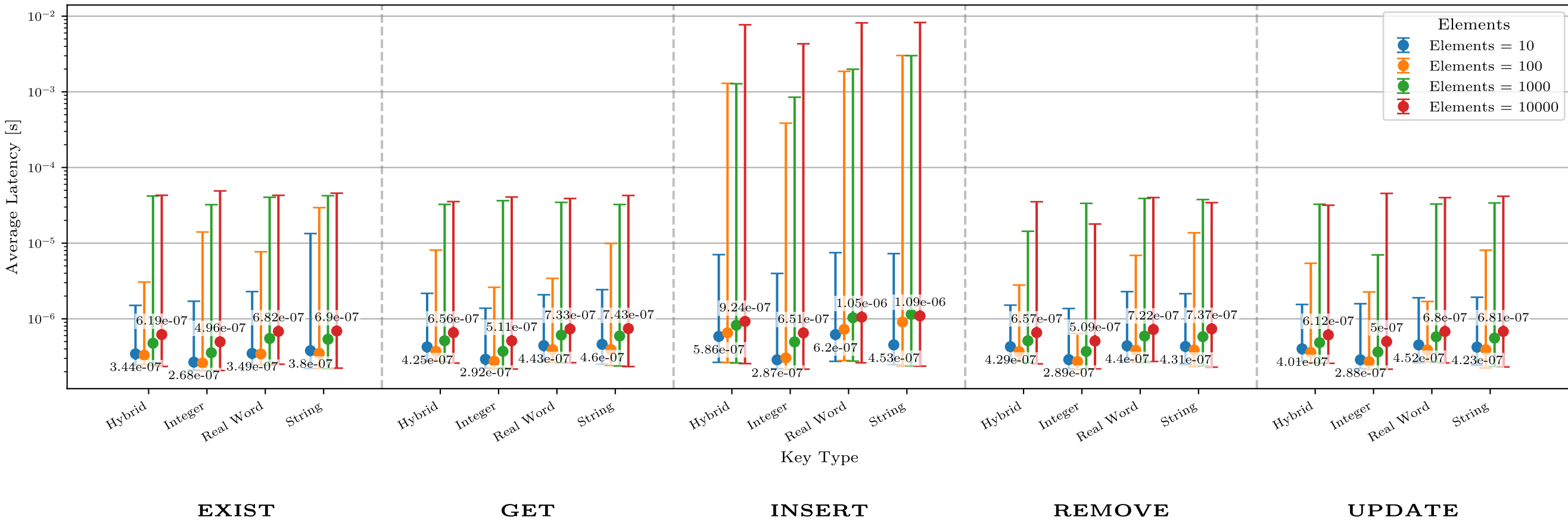
Latency by Operation and Key Type
