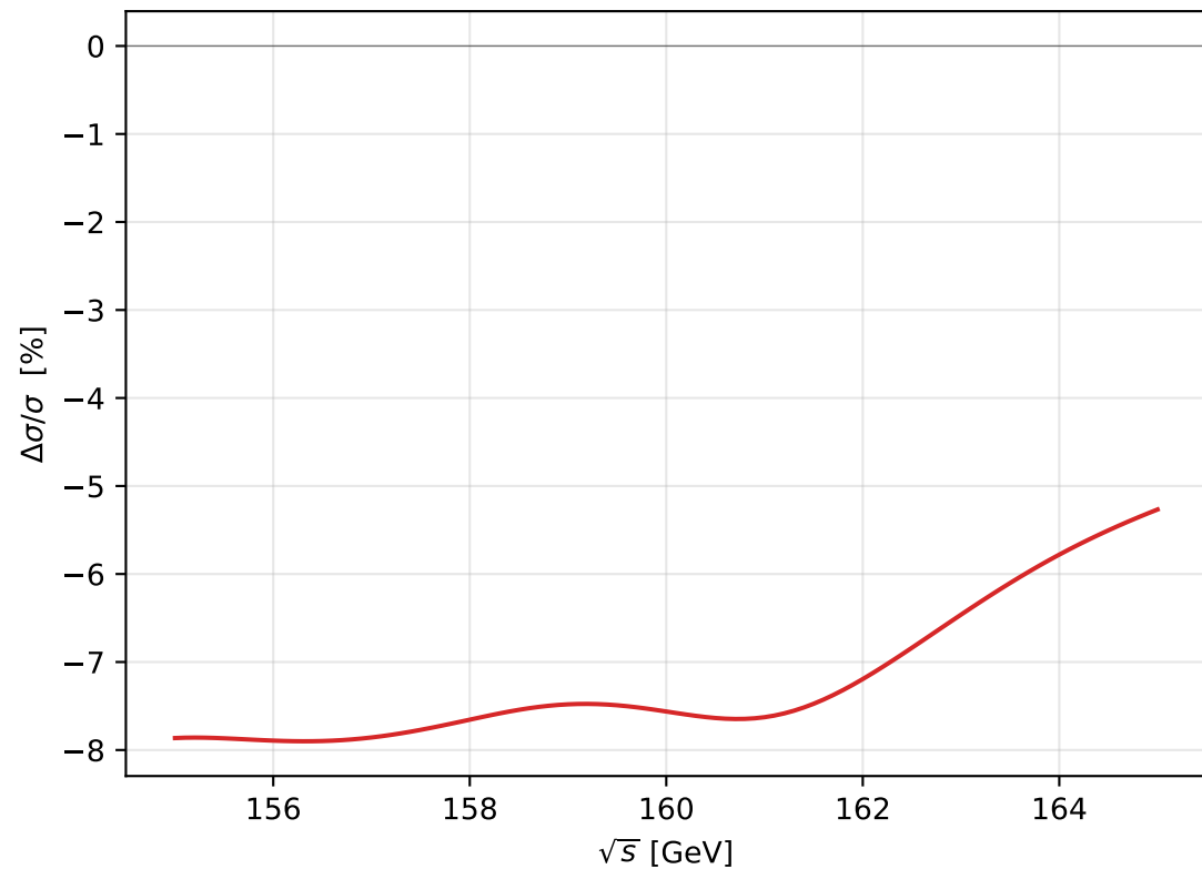
Width sensitivity \partial\sigma/\partial\Gamma_W
