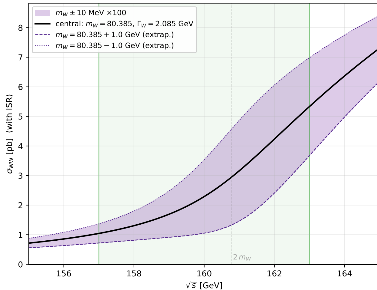
m_W variation ( \pm 1.0 GeV, linear from \pm 10 MeV)
