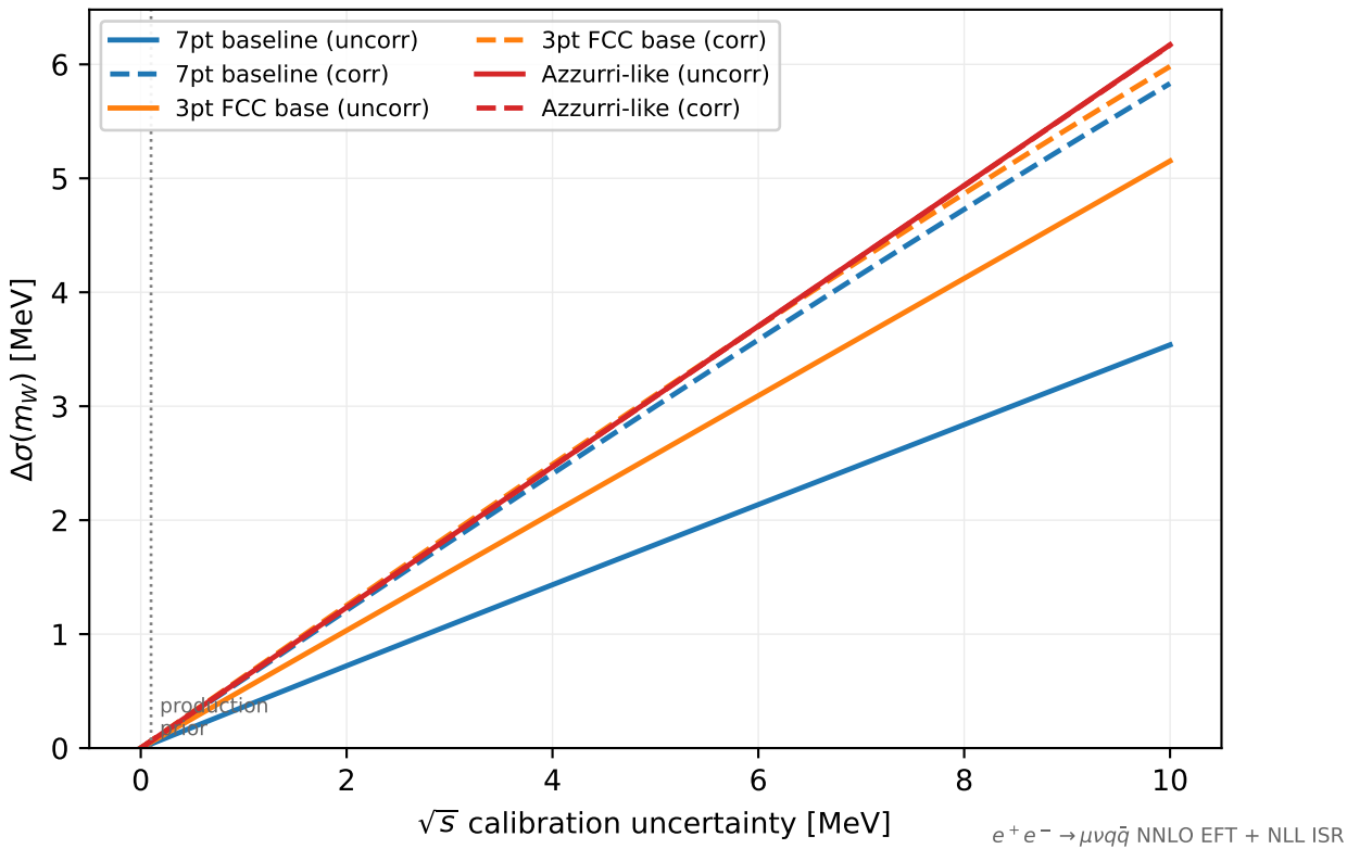
\sigma(m_W) impact vs BEC input across scan scenarios
