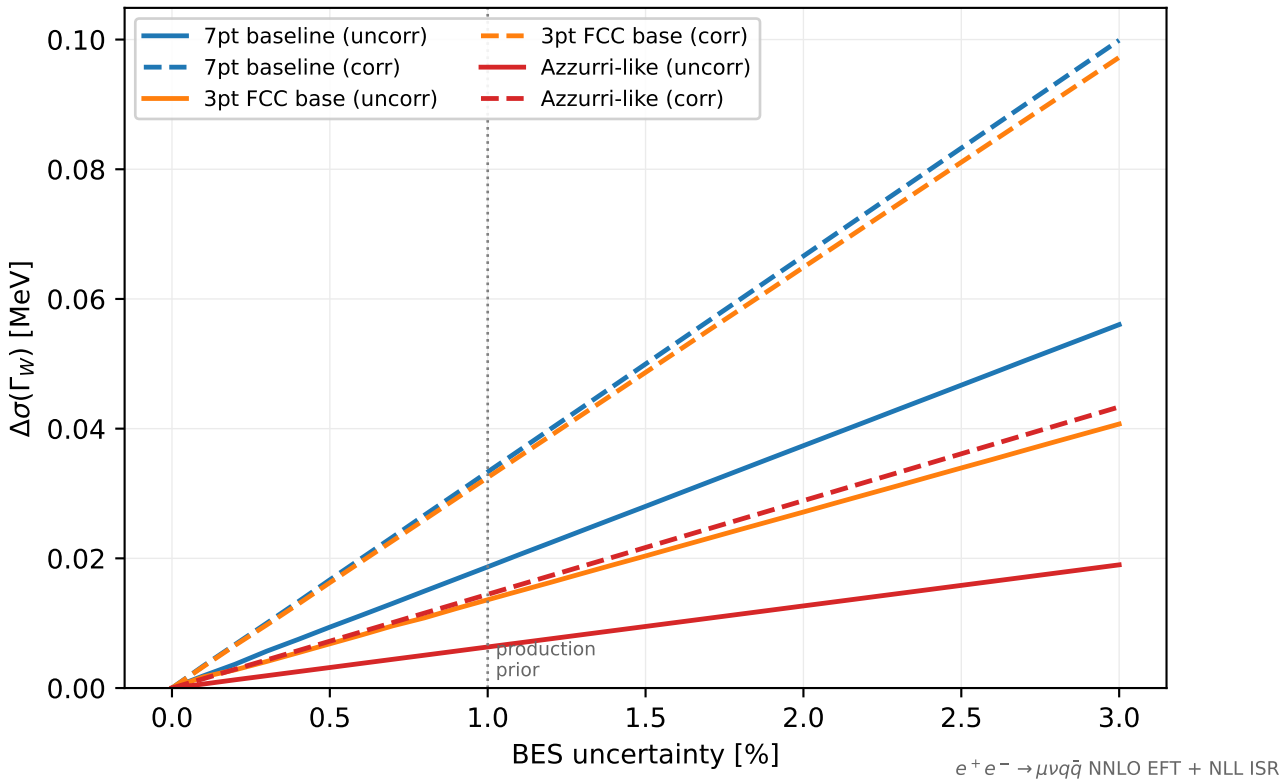
\sigma(\Gamma_W) impact vs BES input across scan scenarios
