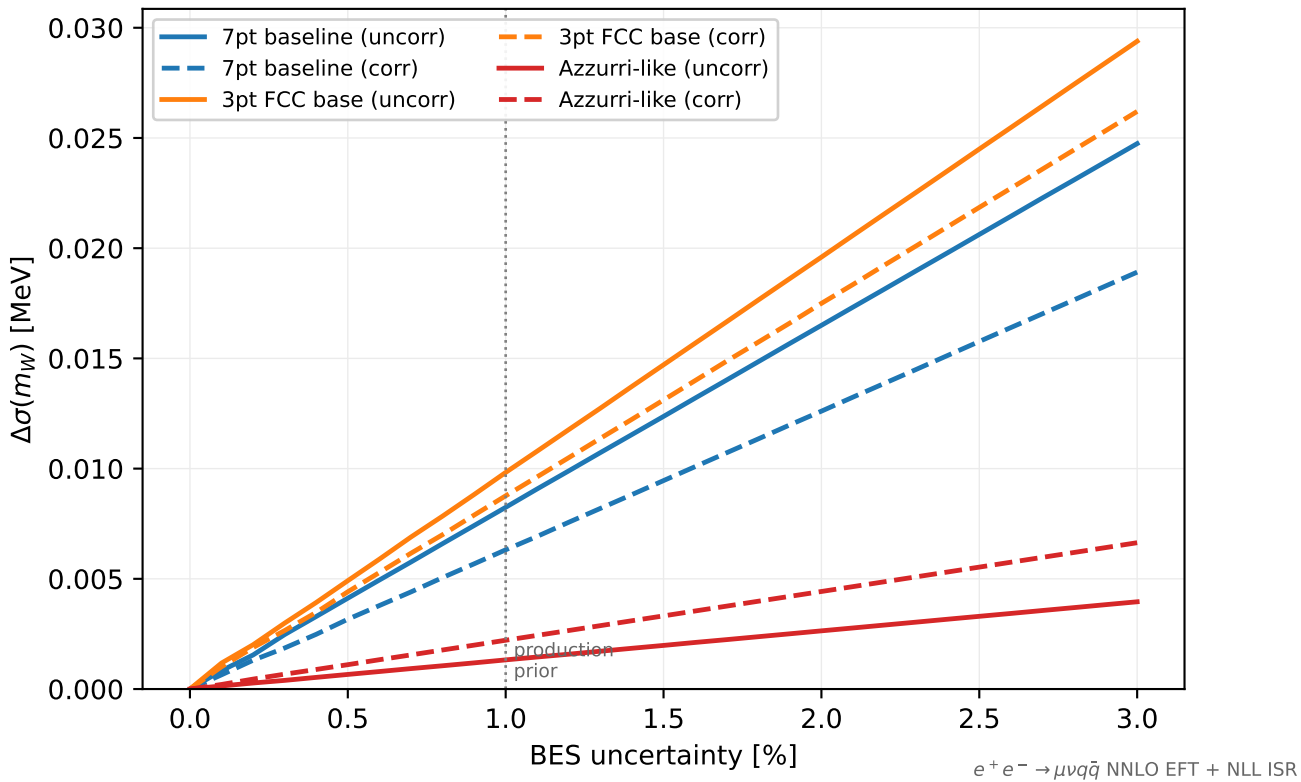
\sigma(m_W) impact vs BES input across scan scenarios
