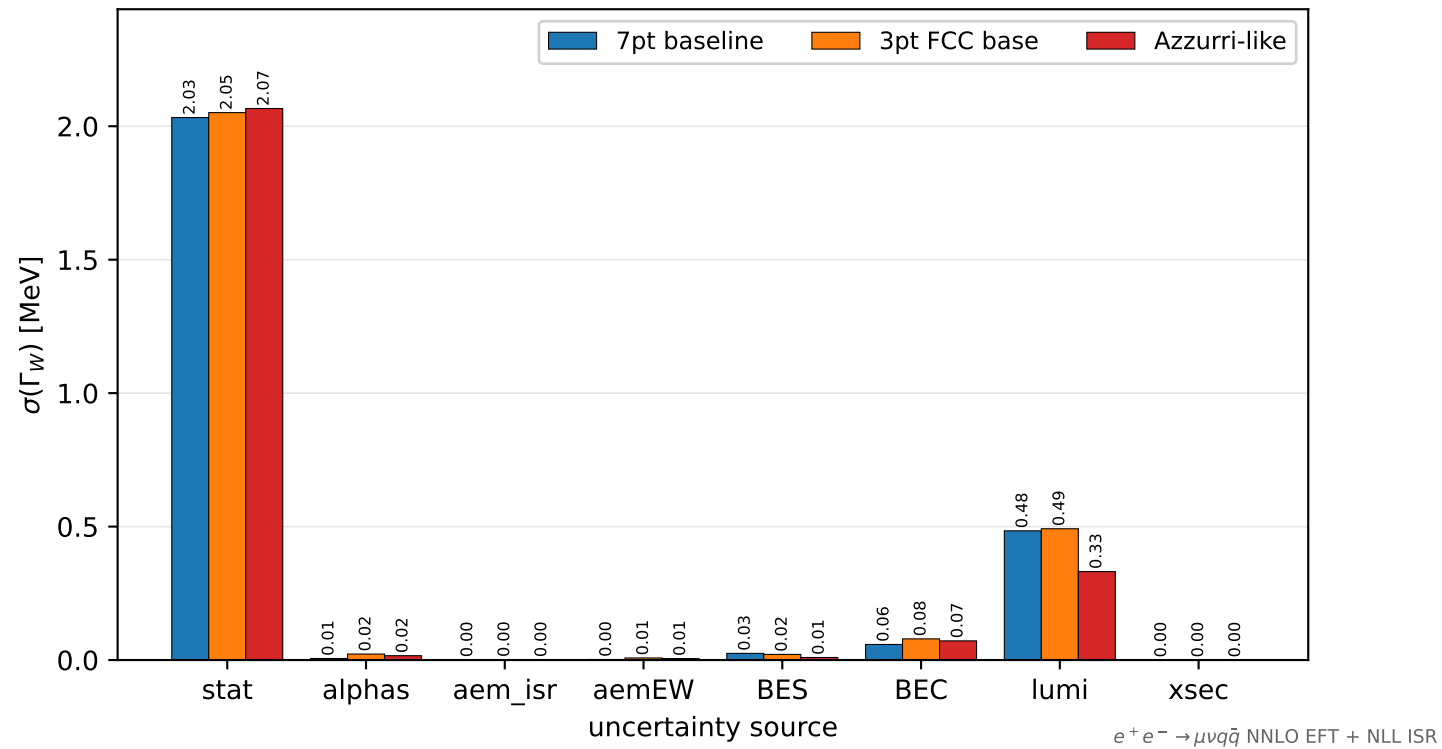
\sigma(\Gamma_W) breakdown across scan scenarios (same 19.2 \text{ ab}^{-1} )
