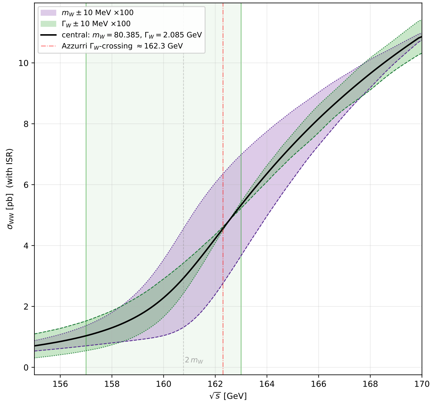
m_W and \Gamma_W \pm 1.0 GeV bands overlaid (linear from \pm 10 MeV, \times 100 )
