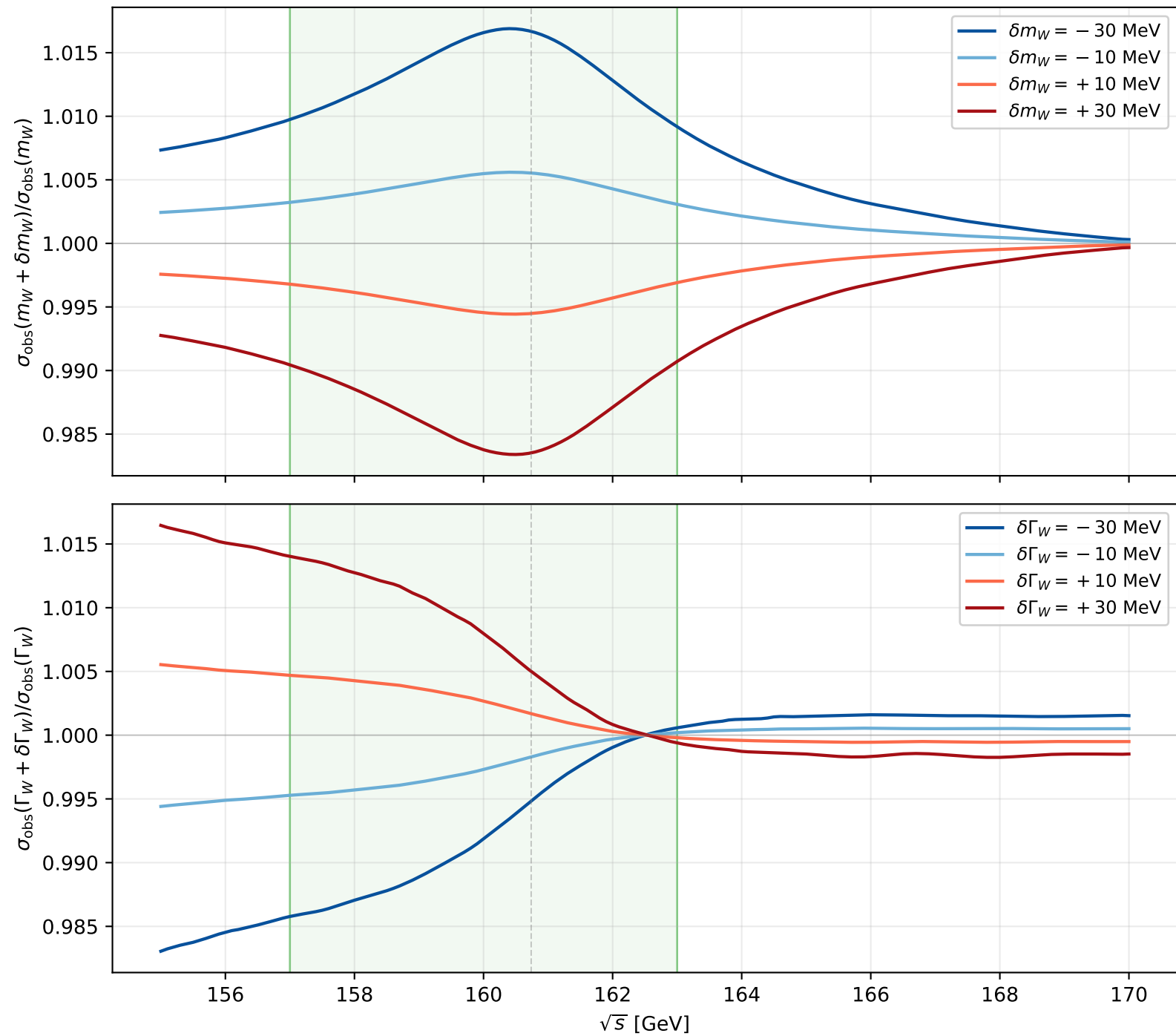
Lineshape sensitivity to m_W and \Gamma_W ( m_W = 80.3692 GeV, \Gamma_W = 2.085 GeV, with ISR)
