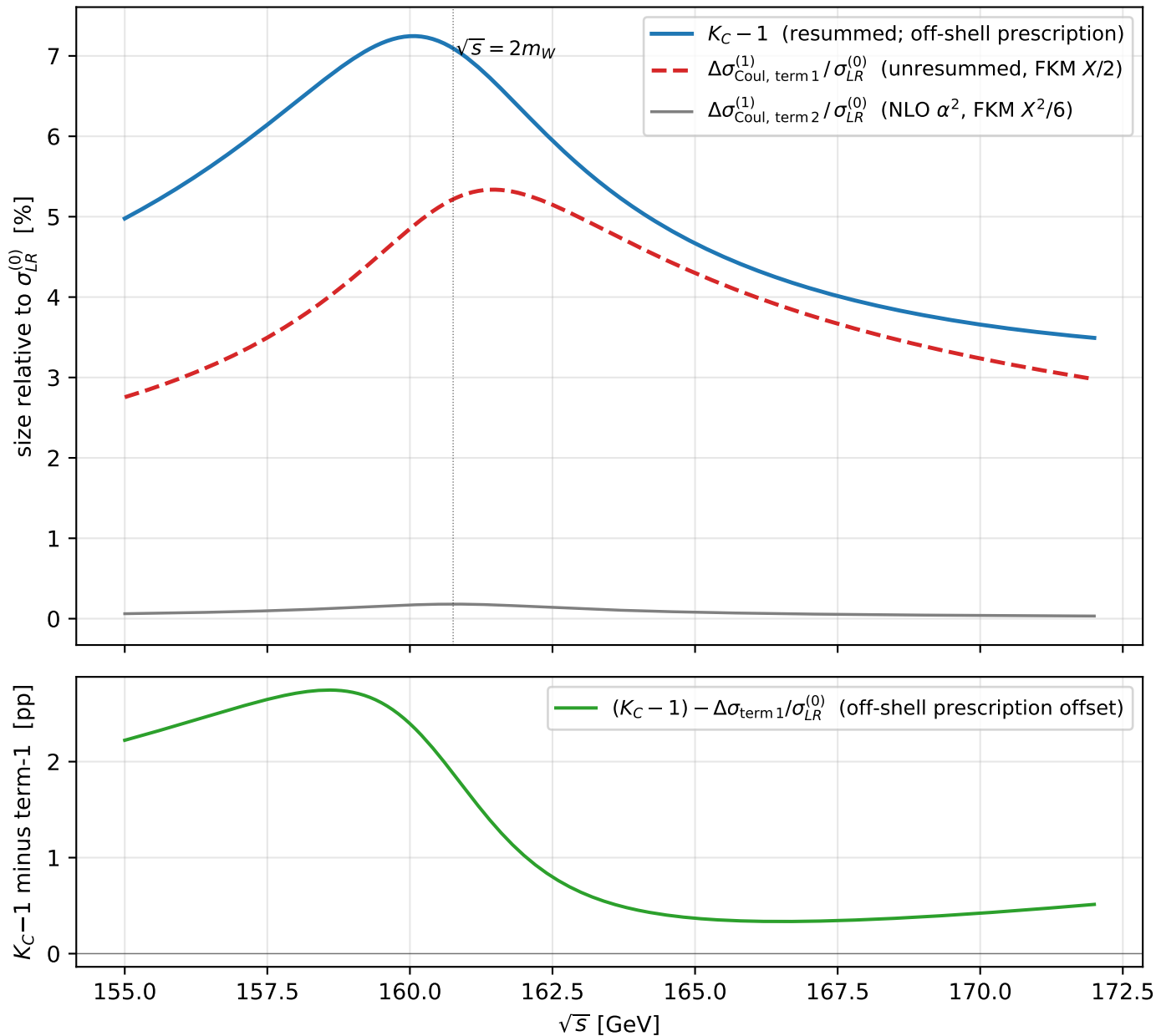
Leading- \alpha/v Coulomb: two formulations of the same physics
