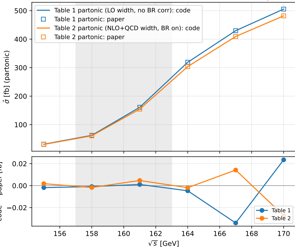
BFS NLO Tables 1 & 2: partonic N^{3/2} LO EFT Born for e^+e^- \rightarrow \mu^- \bar{\nu}_\mu u \bar{d} (no ISR)
