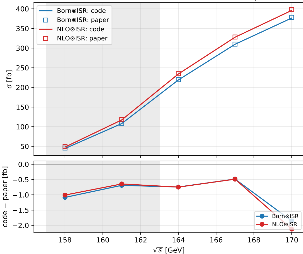
BFS NLO Table 4: Born \otimes ISR and NLO for \mu^- \bar{\nu}_\mu u \bar{d}
