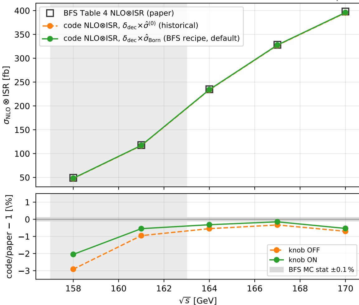
BFS Table~4 NLO \otimes ISR closure: decay substitution A/B ( \mu^- \bar{\nu}_\mu u \bar{d} )
