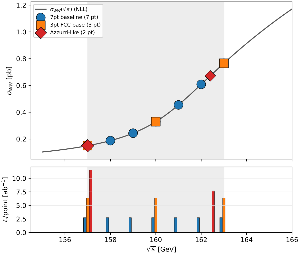
WW threshold scan layouts (same total 19.2 \text{ab}^{-1} )
