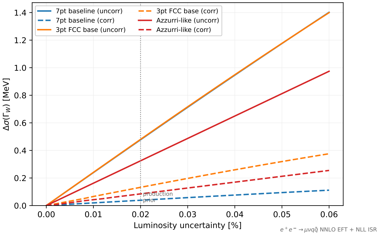
\sigma(\Gamma_W) impact vs lumi input across scan scenarios
