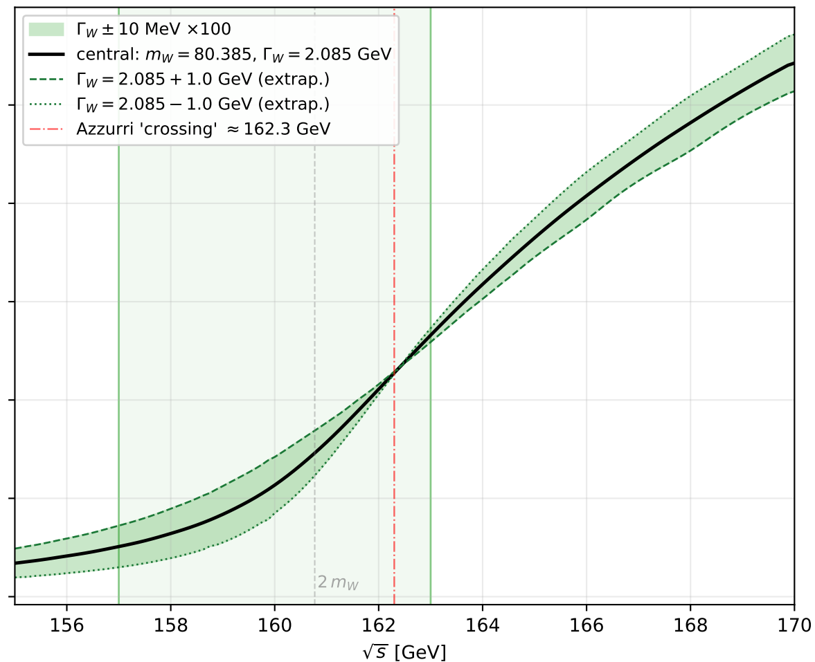
\Gamma_W variation ( \pm 1.0 GeV, linear from \pm 10 MeV)
