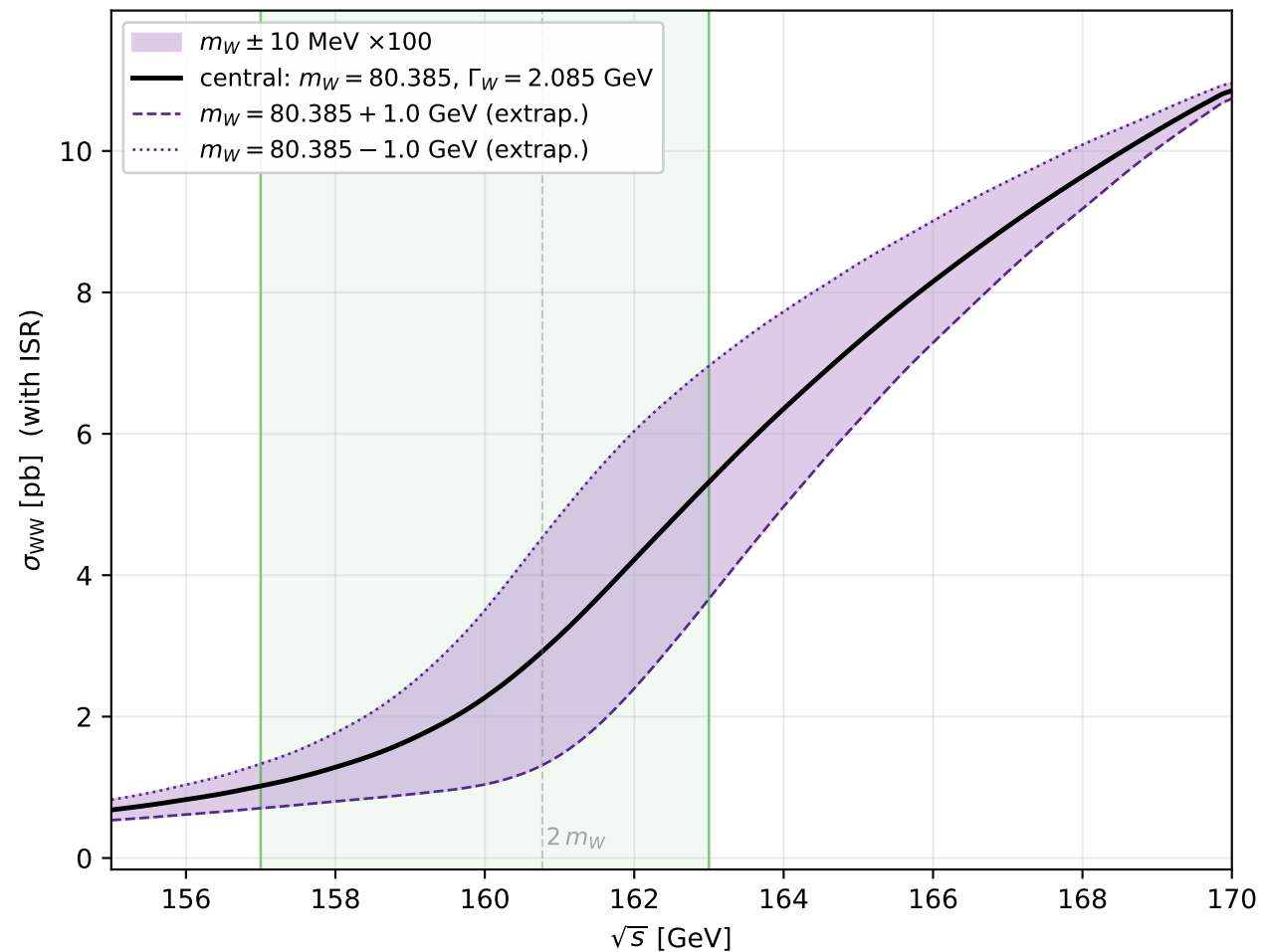
m_W variation ( \pm 1.0 GeV, linear from \pm 10 MeV)
