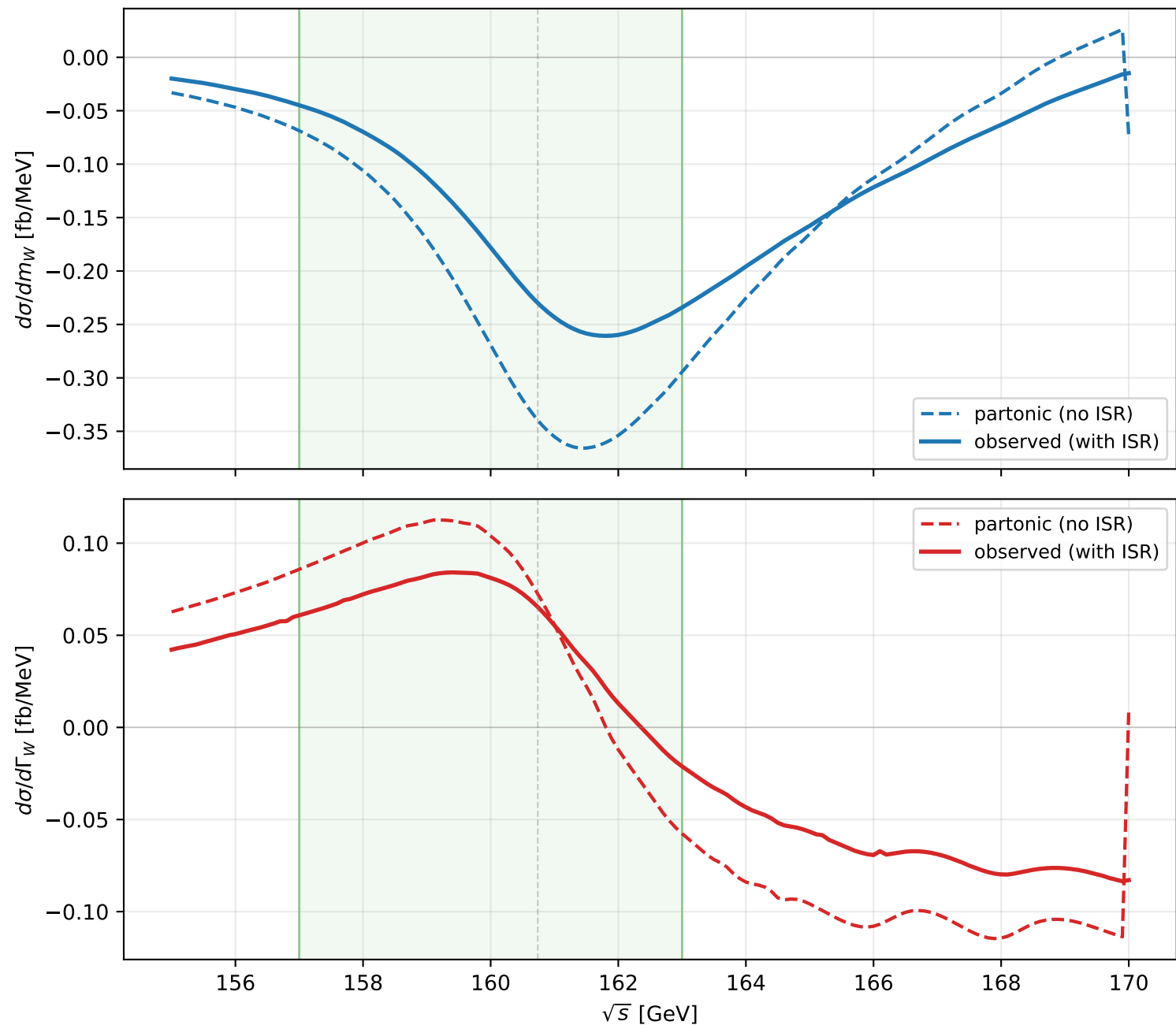
Sensitivity of \sigma(\mu\nu q\bar{q}) to m_W and \Gamma_W ( m_W = 80.3692 GeV, \Gamma_W = 2.085 GeV)
