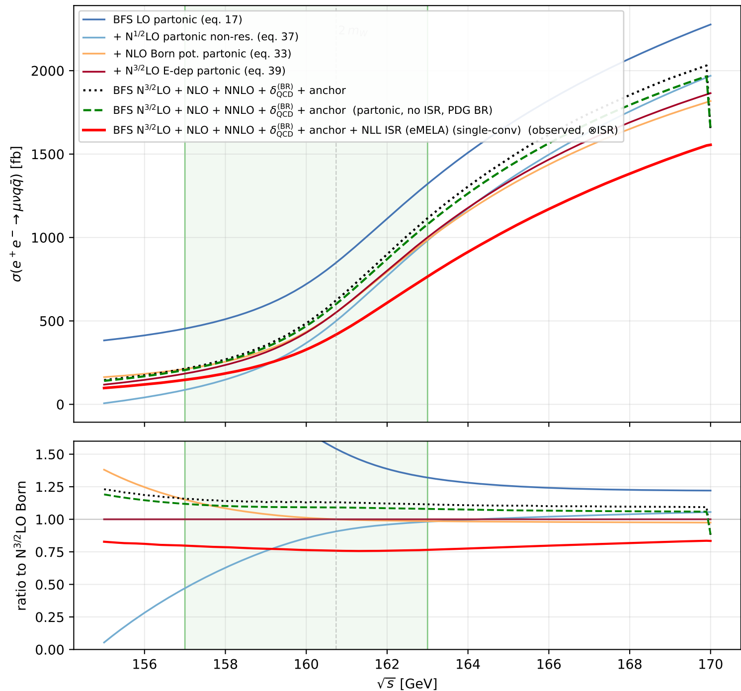
WW threshold cross section vs \sqrt{s} ( m_W = 80.3692 GeV, \Gamma_W = 2.085 GeV)
