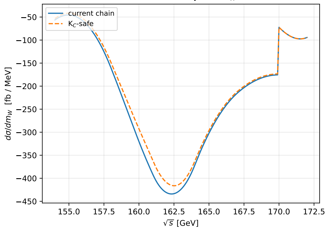
Mass sensitivity \partial\sigma/\partial m_W
