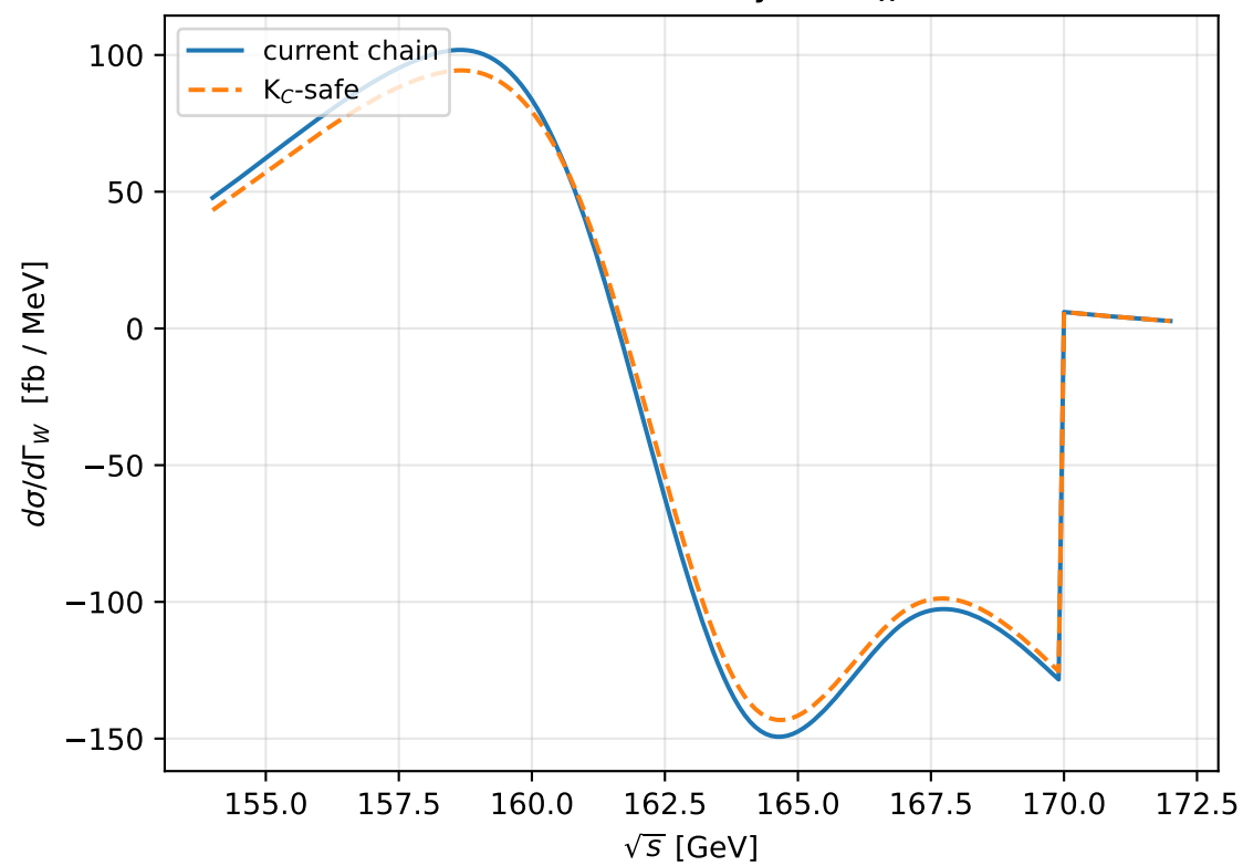
Width sensitivity \partial\sigma/\partial\Gamma_W
