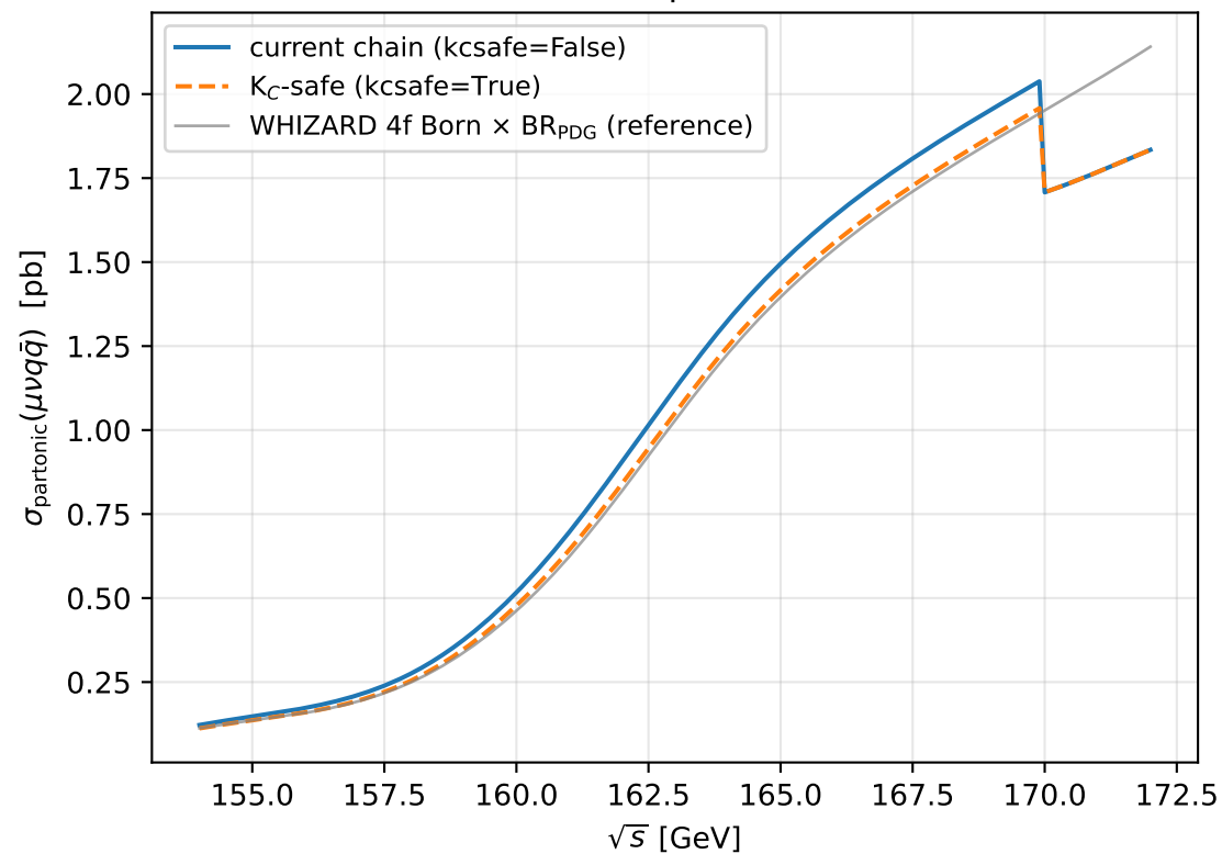
Absolute partonic \sigma
