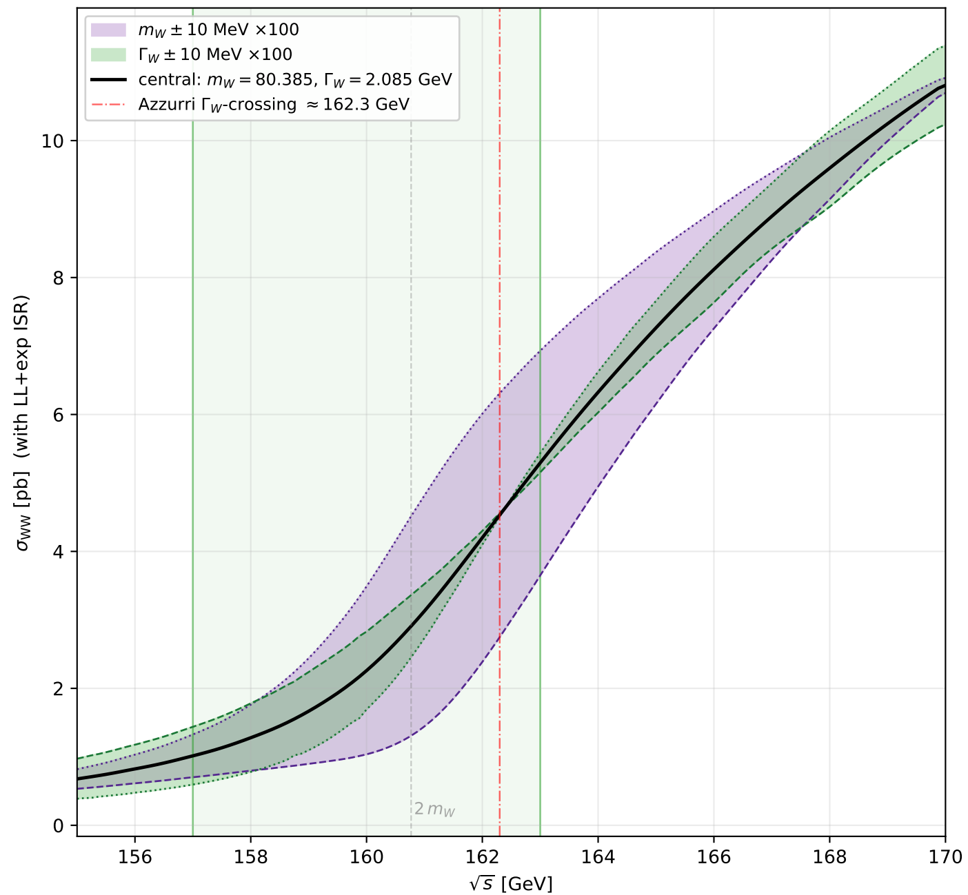
m_W and \Gamma_W \pm 1.0 GeV bands overlaid (linear from \pm 10 MeV, \times 100 )
