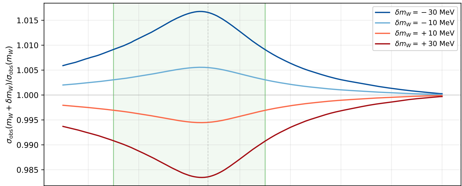
Lineshape sensitivity to m_W and \Gamma_W ( m_W = 80.3692 GeV, \Gamma_W = 2.085 GeV, with LL+exp ISR)
