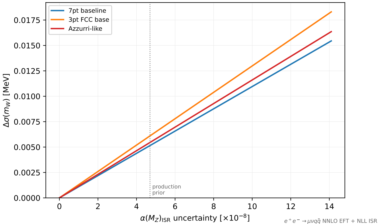
\sigma(m_W) impact vs aem_isr input across scan scenarios
