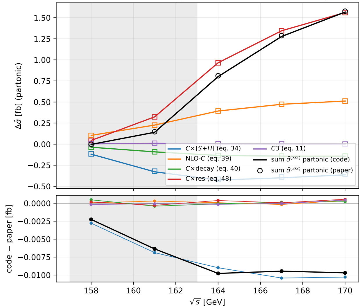
BFS NNLO Table 1: closed-form partonic pieces (helicity-averaged, no ISR)
