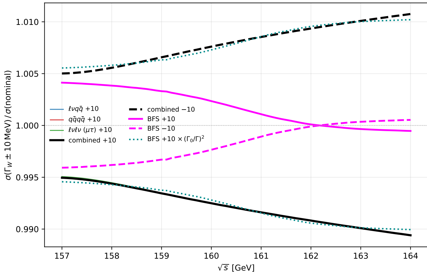
Independent WW vs BFS (off-shell): \Gamma_W response of the line shape
