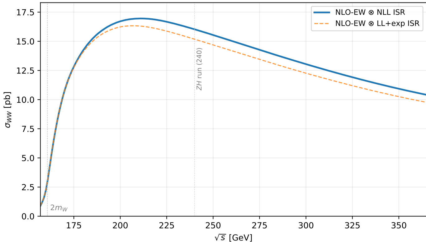
Independent MoCaNLO pure-WW line shape, \sqrt{s} = 157\text{--}365 GeV
