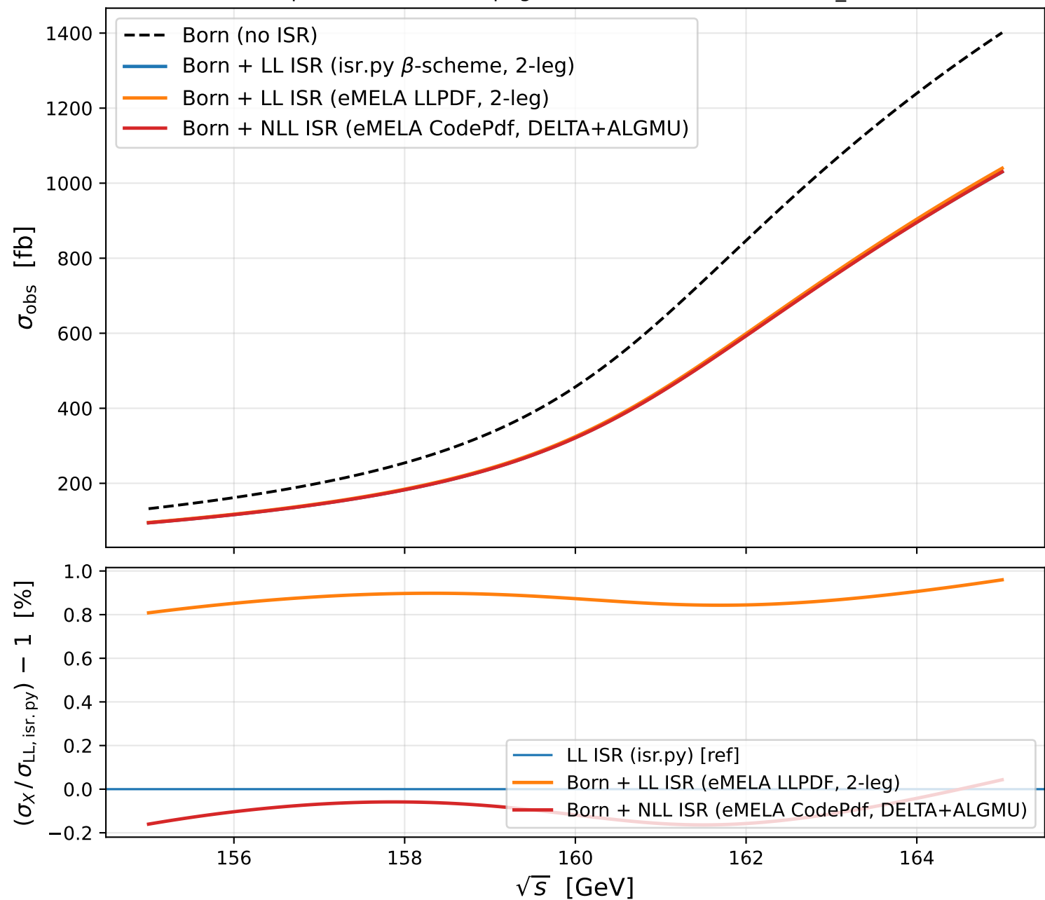
e^+e^- \rightarrow \mu\nu q\bar{q} : ISR scheme comparison (Born-level partonic; inclusive; pdg-constant BR; no NLO/NNLO/ \delta_{\text{QCD}} /anchor)
