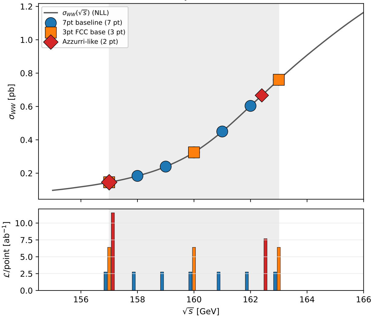
WW threshold scan layouts (same total 19.2 \text{ ab}^{-1} )
