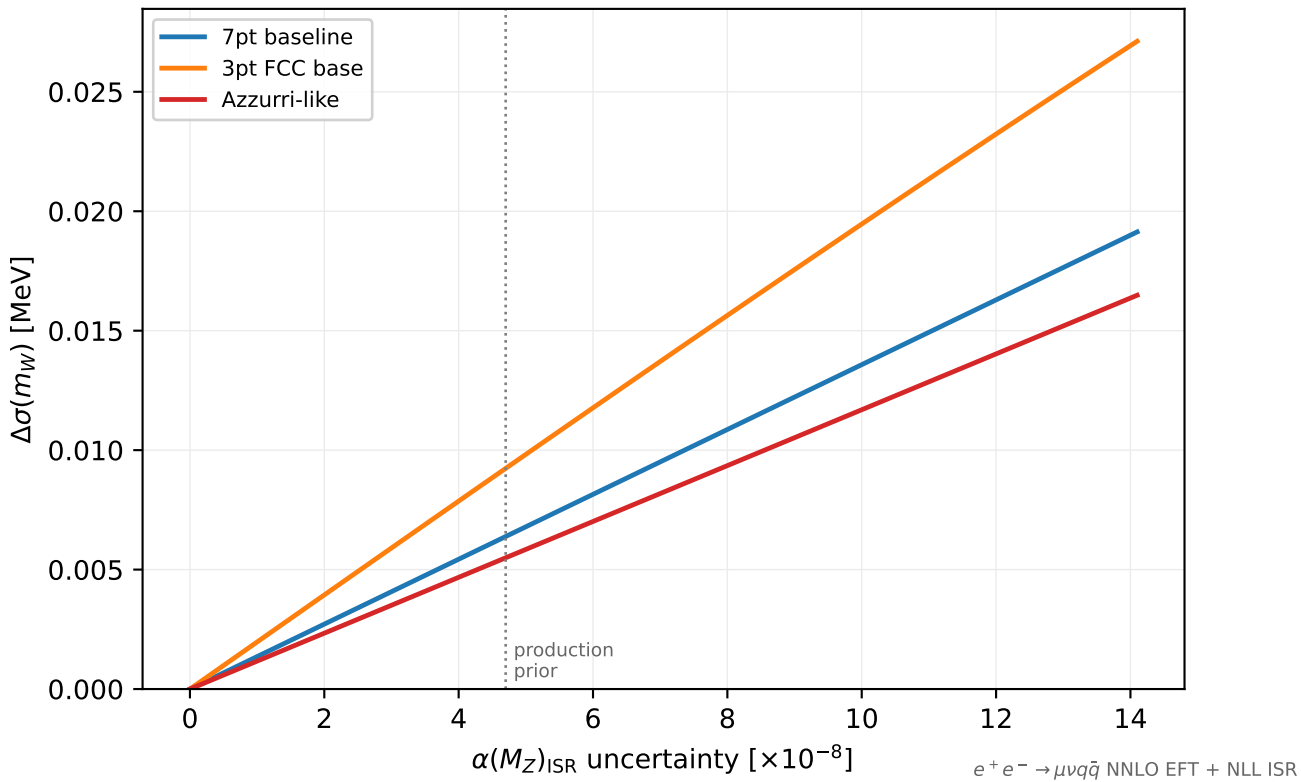
\sigma(m_W) impact vs \alpha_{\text{em}}^{\text{ISR}} input across scan scenarios
