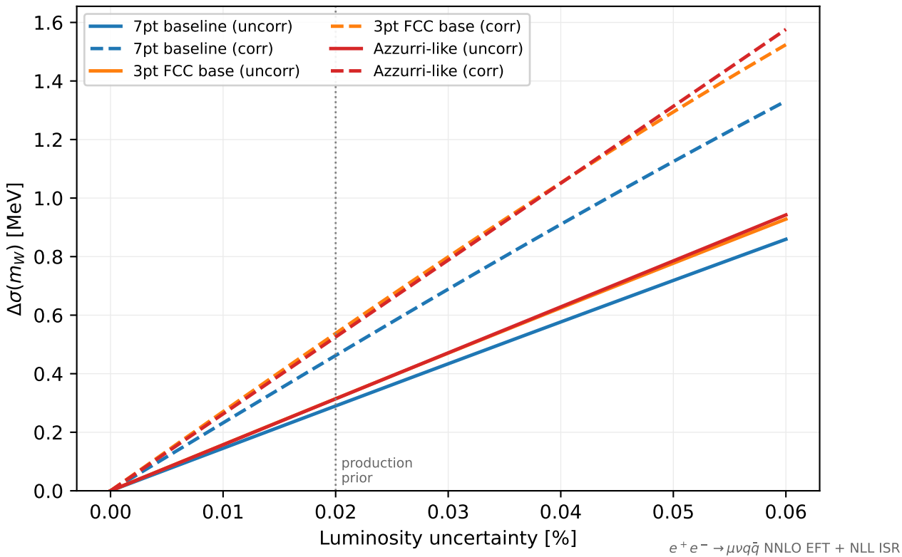
\sigma(m_W) impact vs lumi input across scan scenarios
