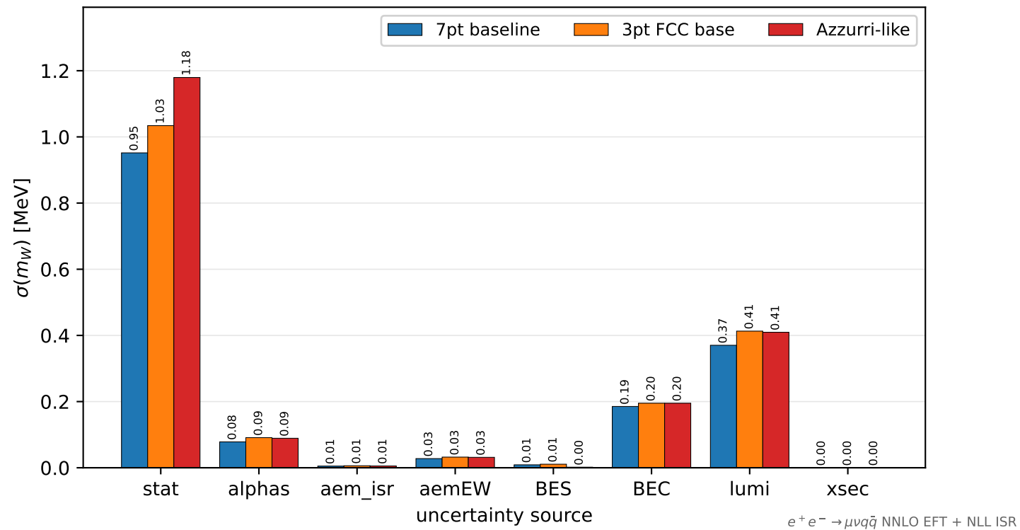
\sigma(m_W) breakdown across scan scenarios (same 19.2 \text{ab}^{-1} )
