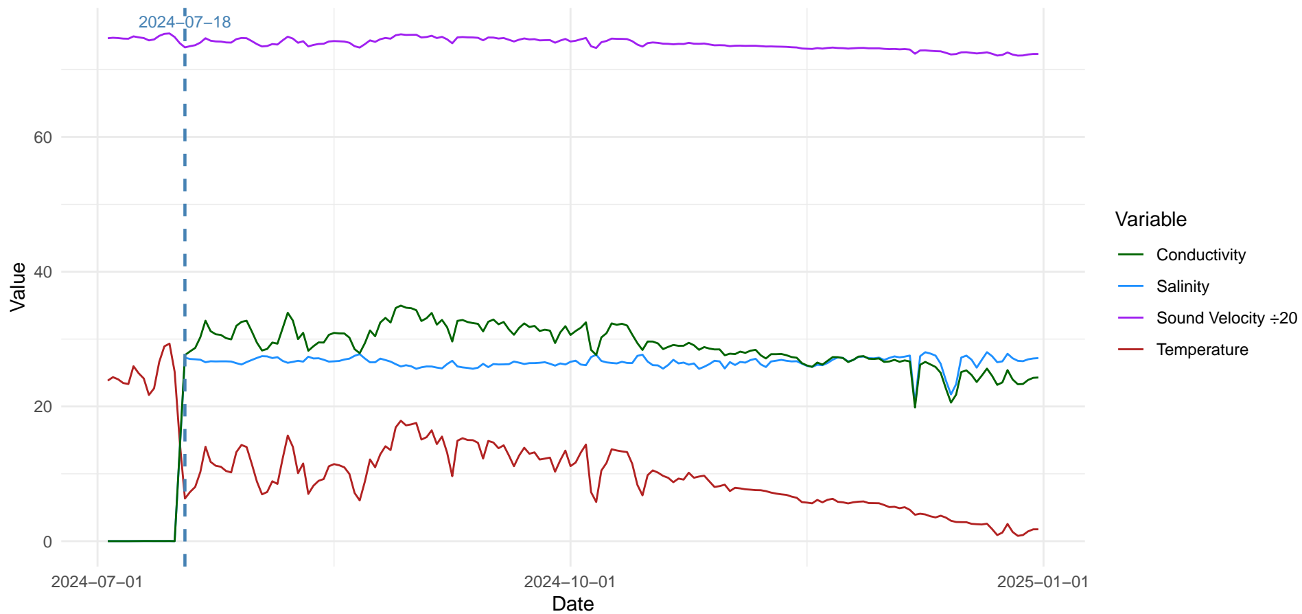
Daily Averages — Site: Anse Bleue 2, NB Probe: s12347
