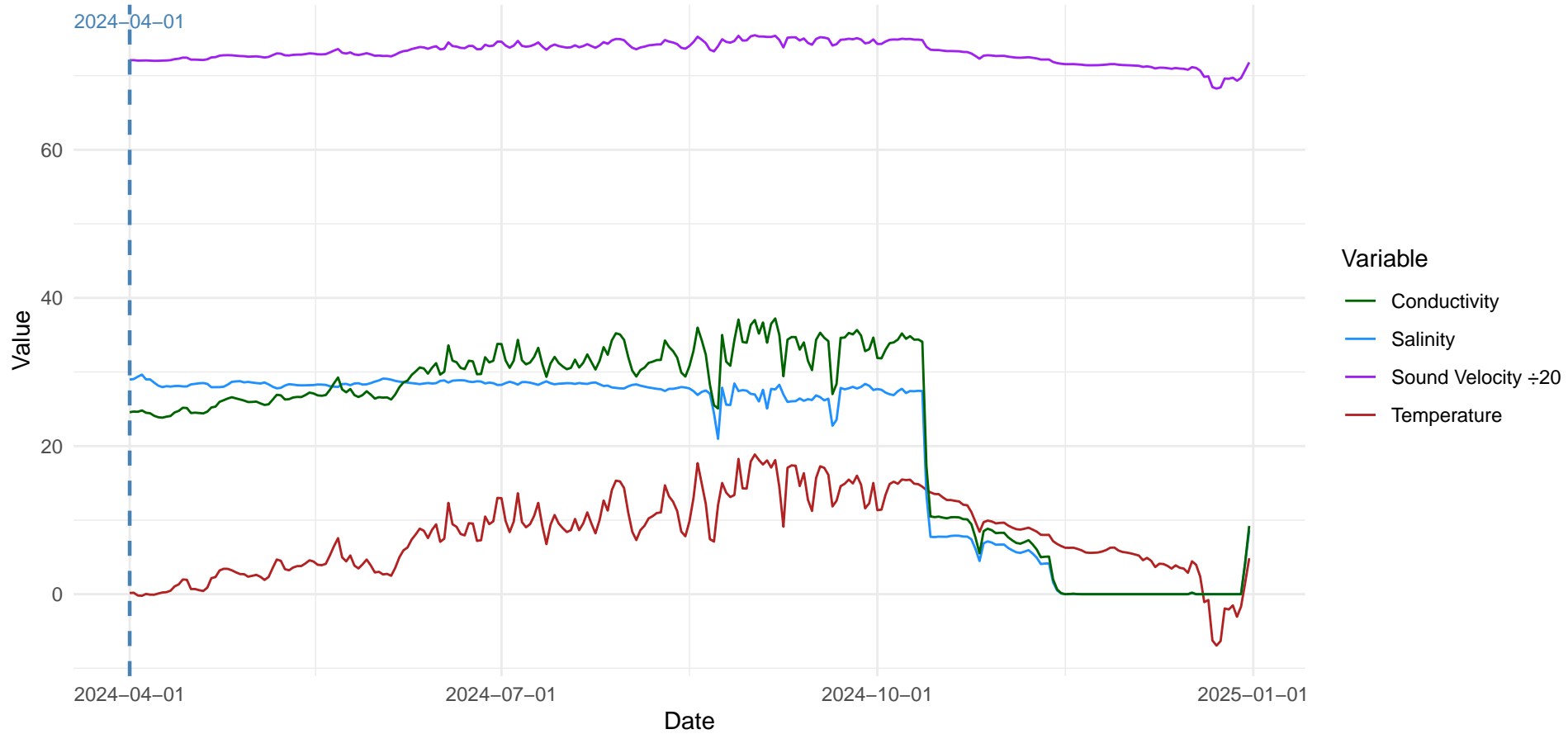
Daily Averages — Site: North Cape, PEI Probe: s11191
