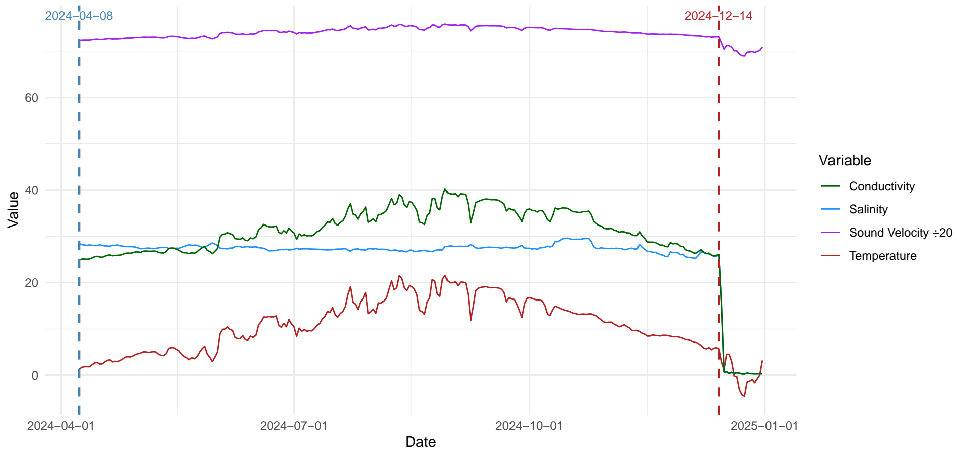
Daily Averages — Site: Jack Shoal, NS Probe: s12333
