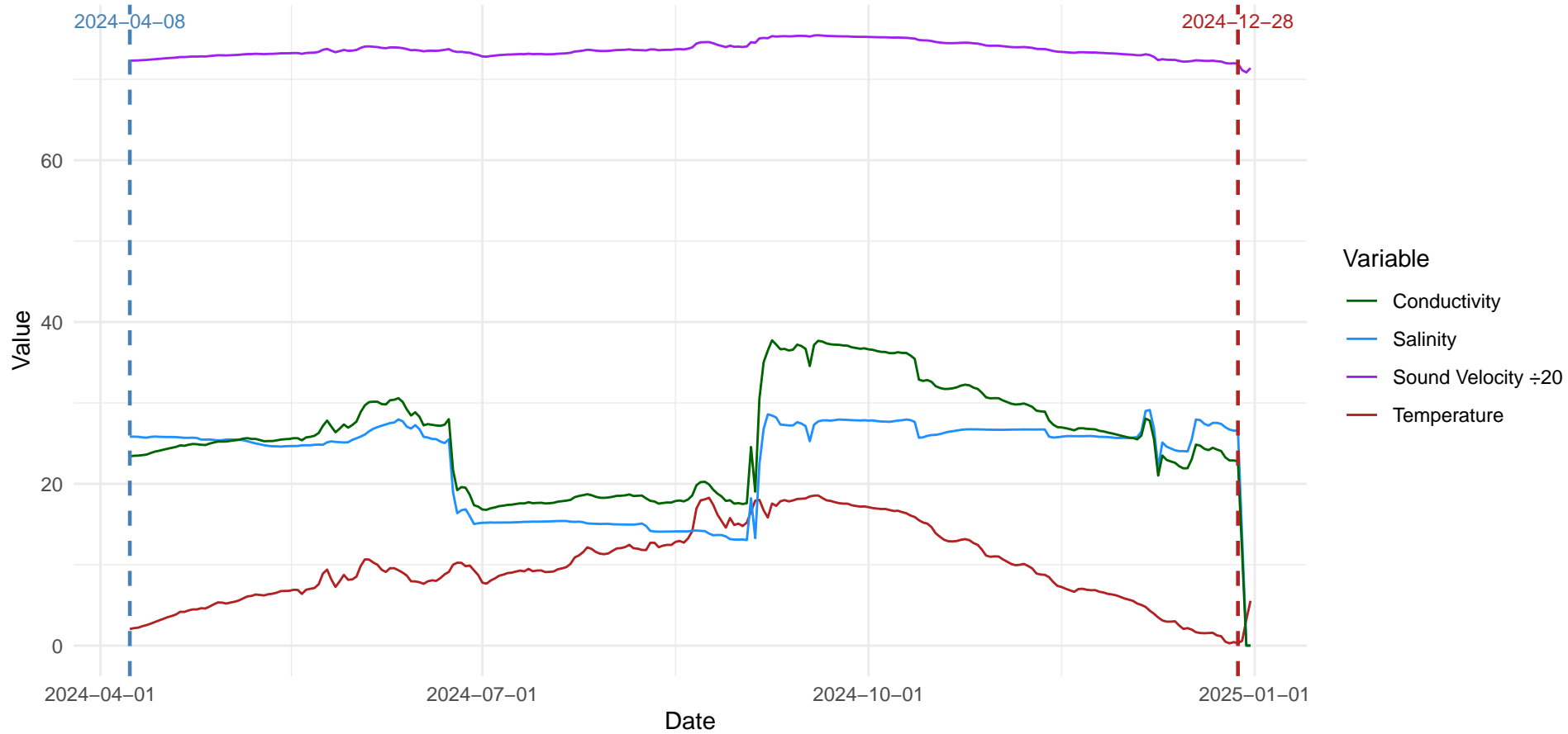
Daily Averages — Site: Strait Crossing 2 Probe: s12342
