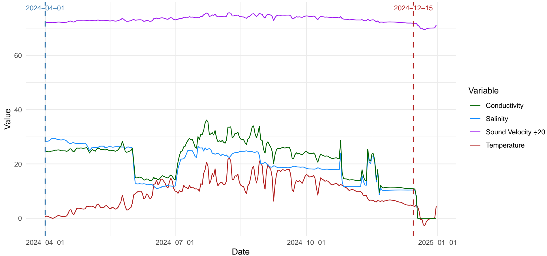
Daily Averages — Site: North Tracadie, PEI Probe: s11192
