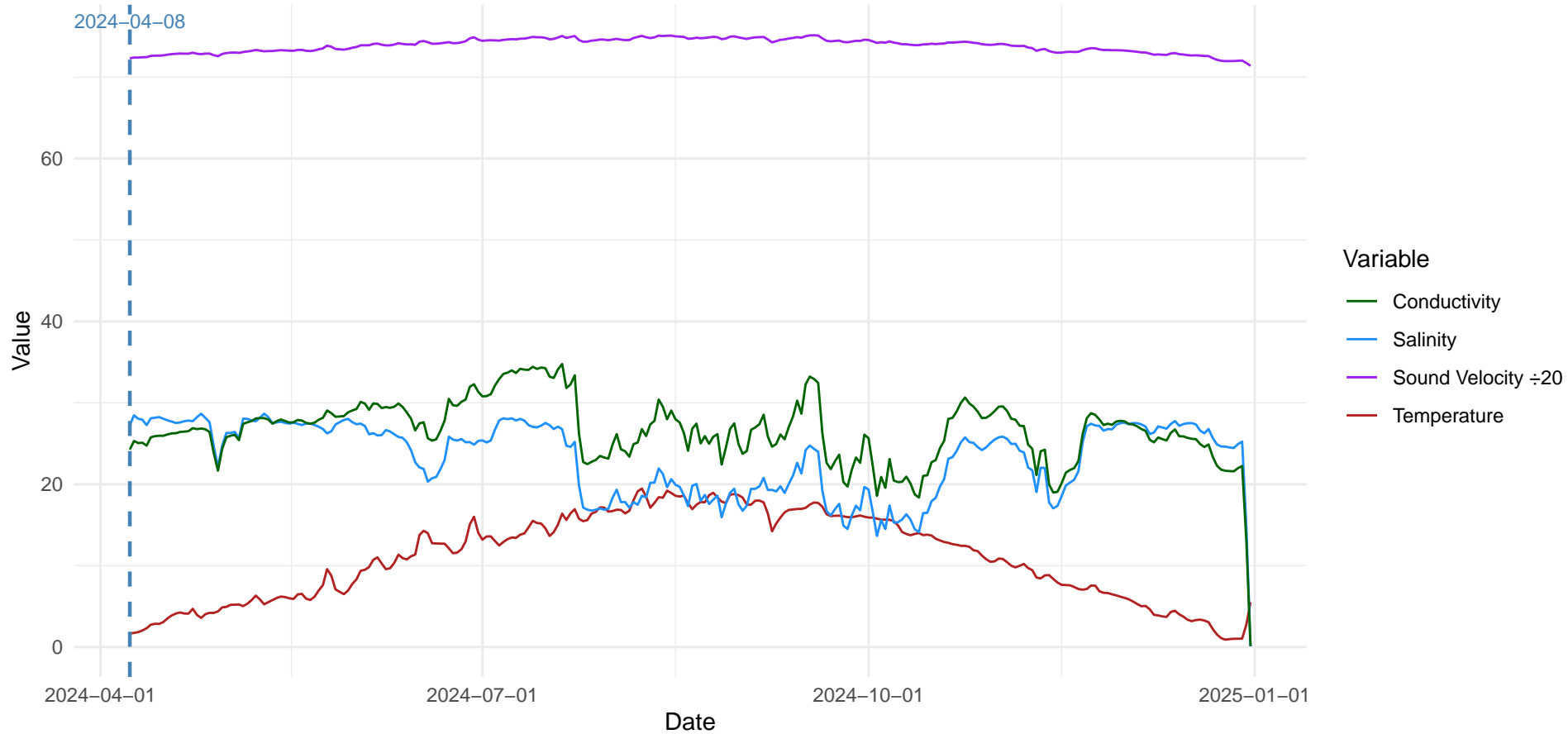
Daily Averages — Site: Caribou, NS Probe: s12304
