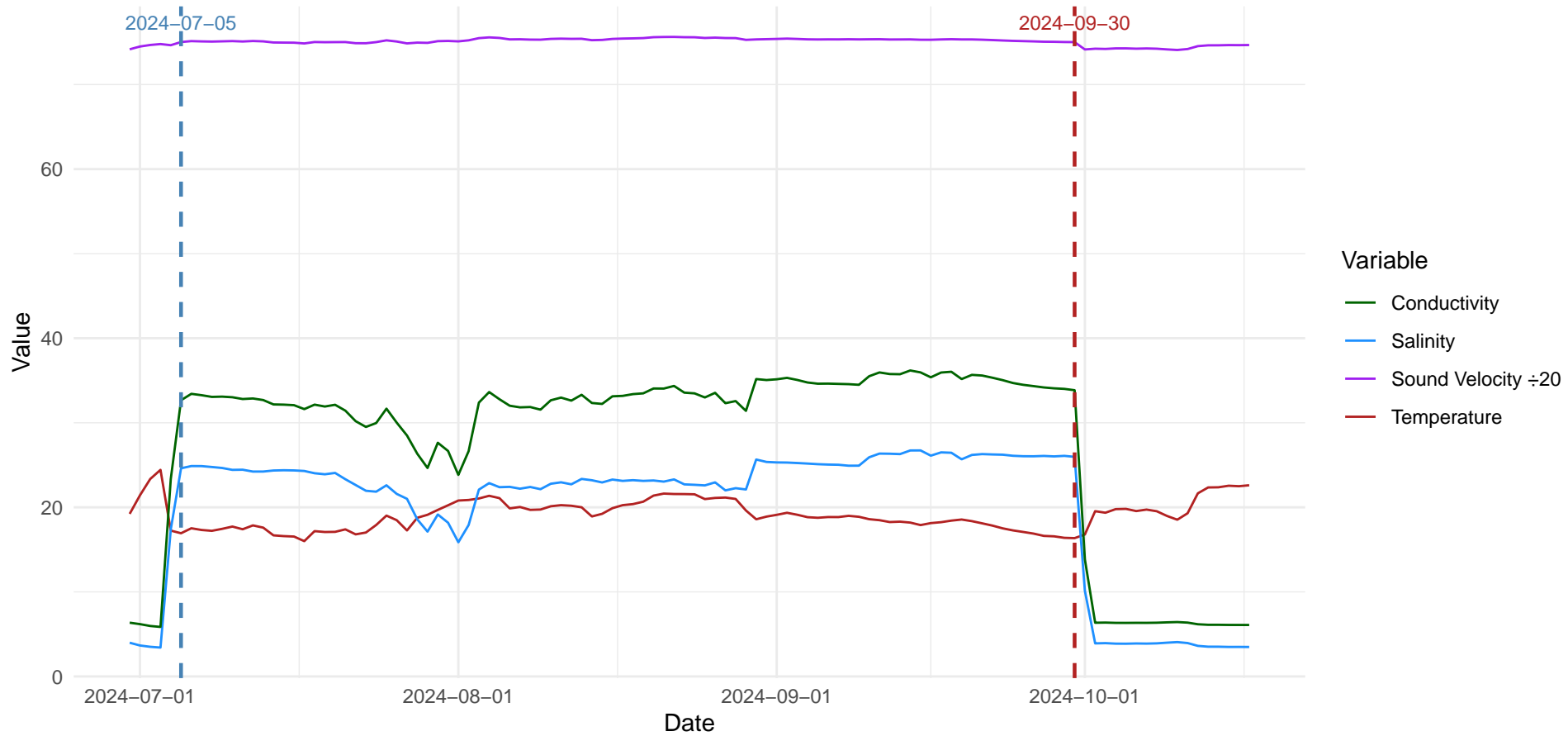
Daily Averages — Site: Nine Mile Creek 2, PEI Probe: s11874
