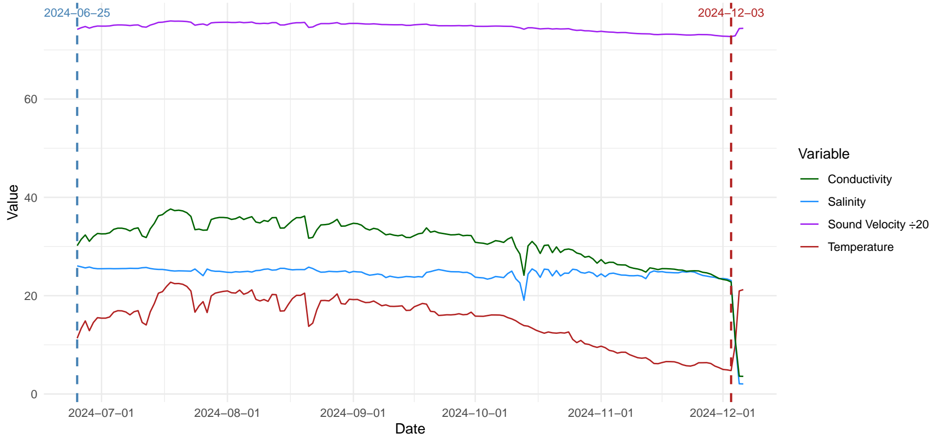
Daily Averages — Site: Skinners Pond, PEI Probe: s11844
