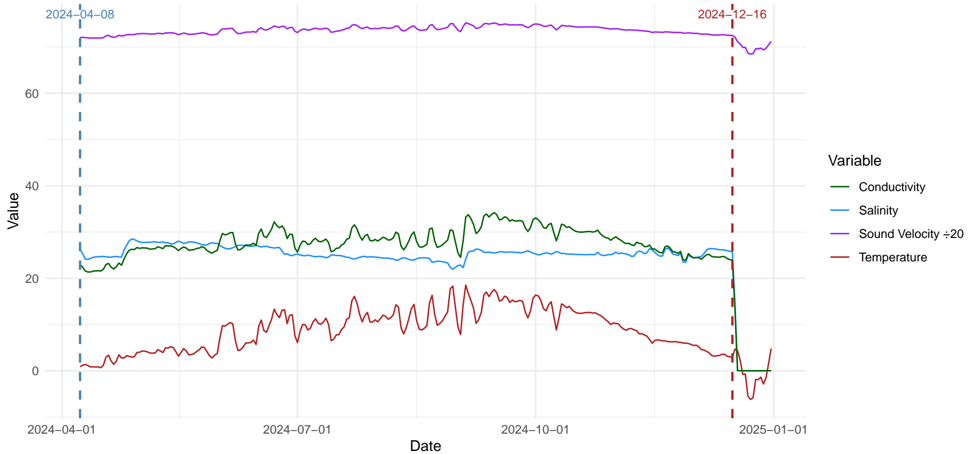
Daily Averages — Site: Malpeque, PEI Probe: s12334
