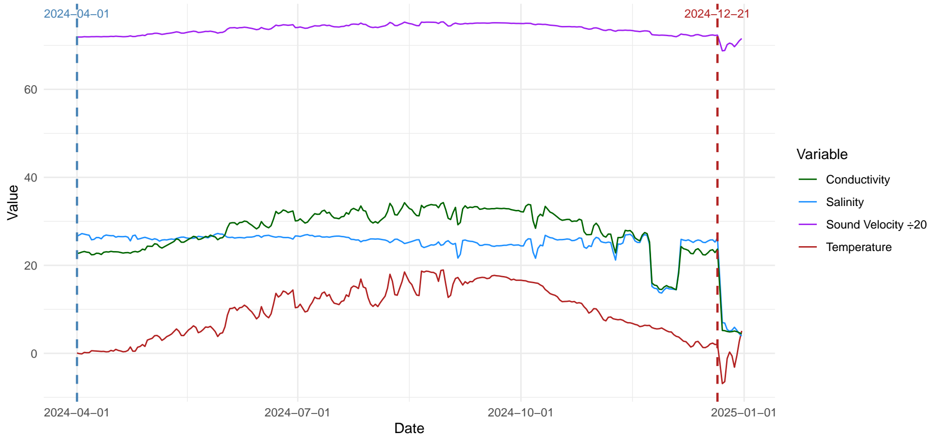
Daily Averages — Site: Pointe Sapin, NB Probe: s11424
