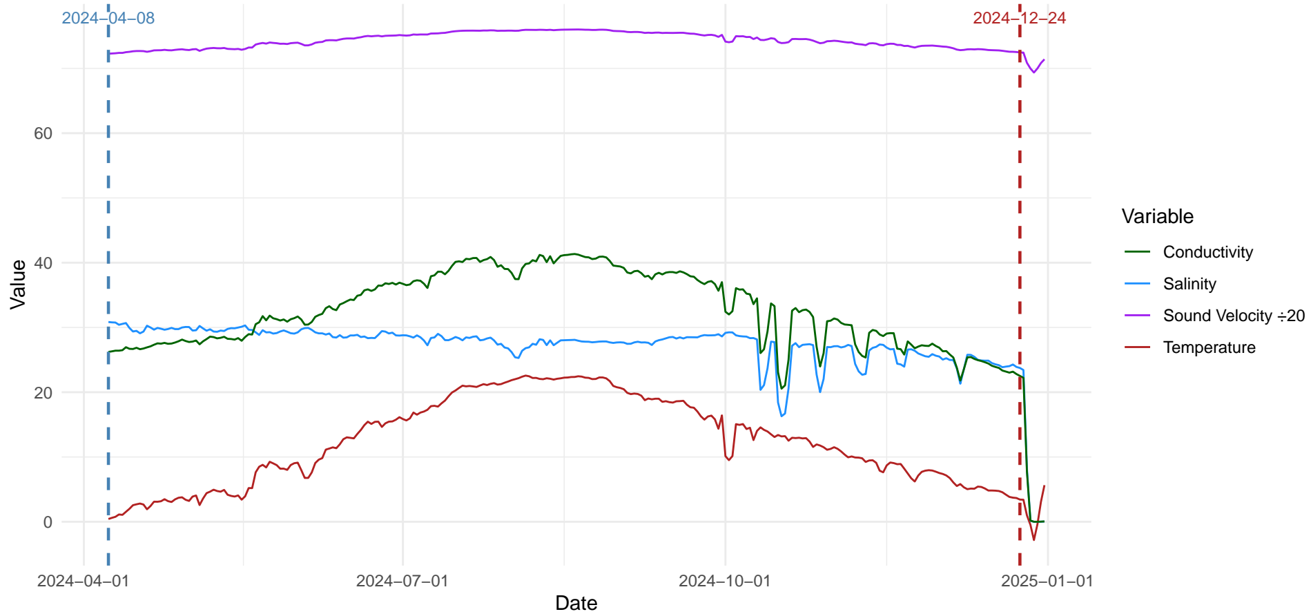
Daily Averages — Site: Pleasant Bay 2, NS Probe: s12339
