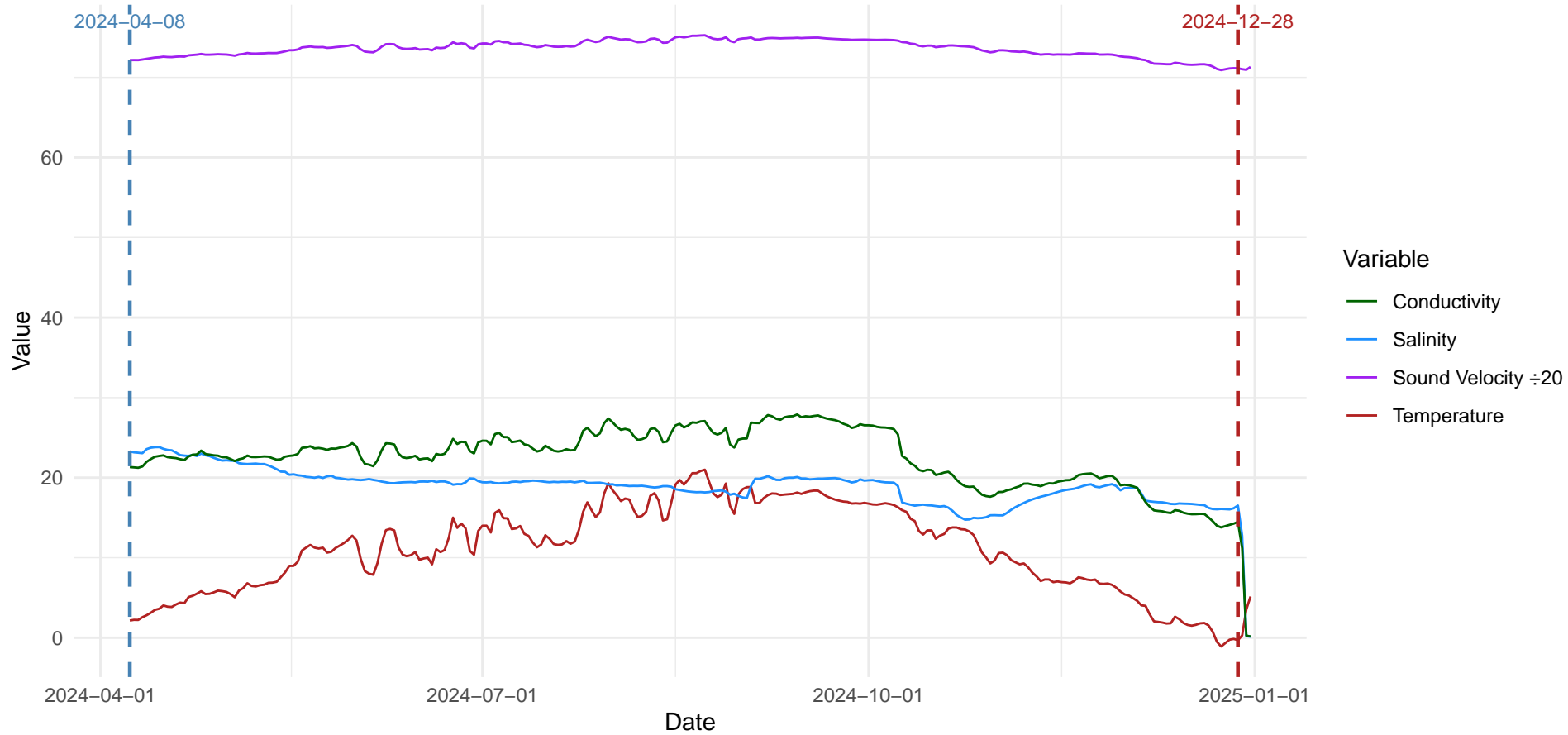
Daily Averages — Site: Victoria, PEI Probe: s12345
