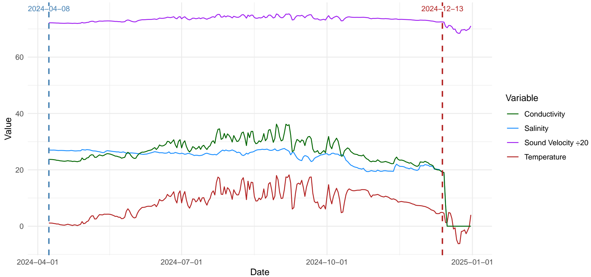
Daily Averages — Site: Souris, PEI Probe: s12341
