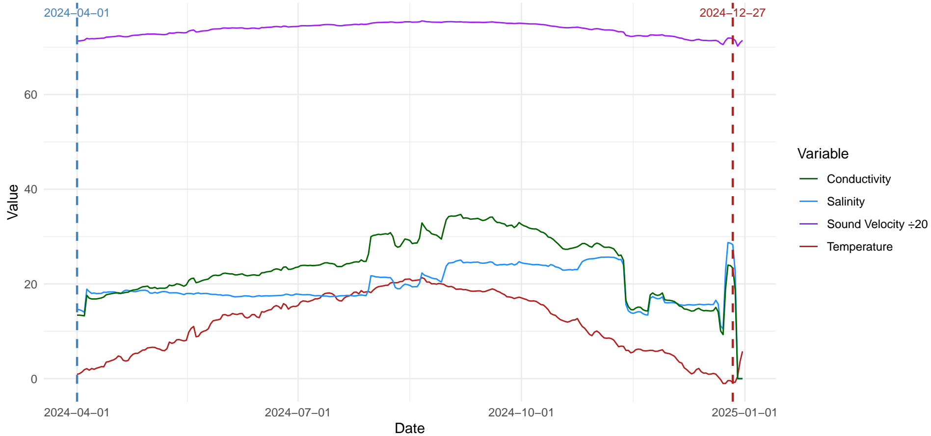
Daily Averages — Site: Shediac, NB Probe: s11194
