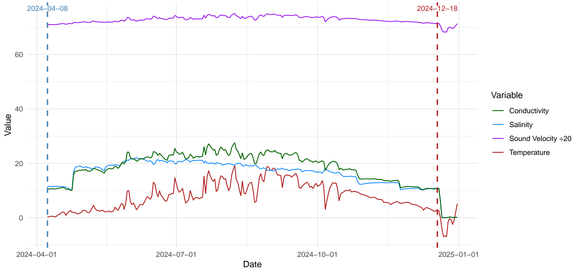
Daily Averages — Site: Shippagan, NB Probe: s12340
