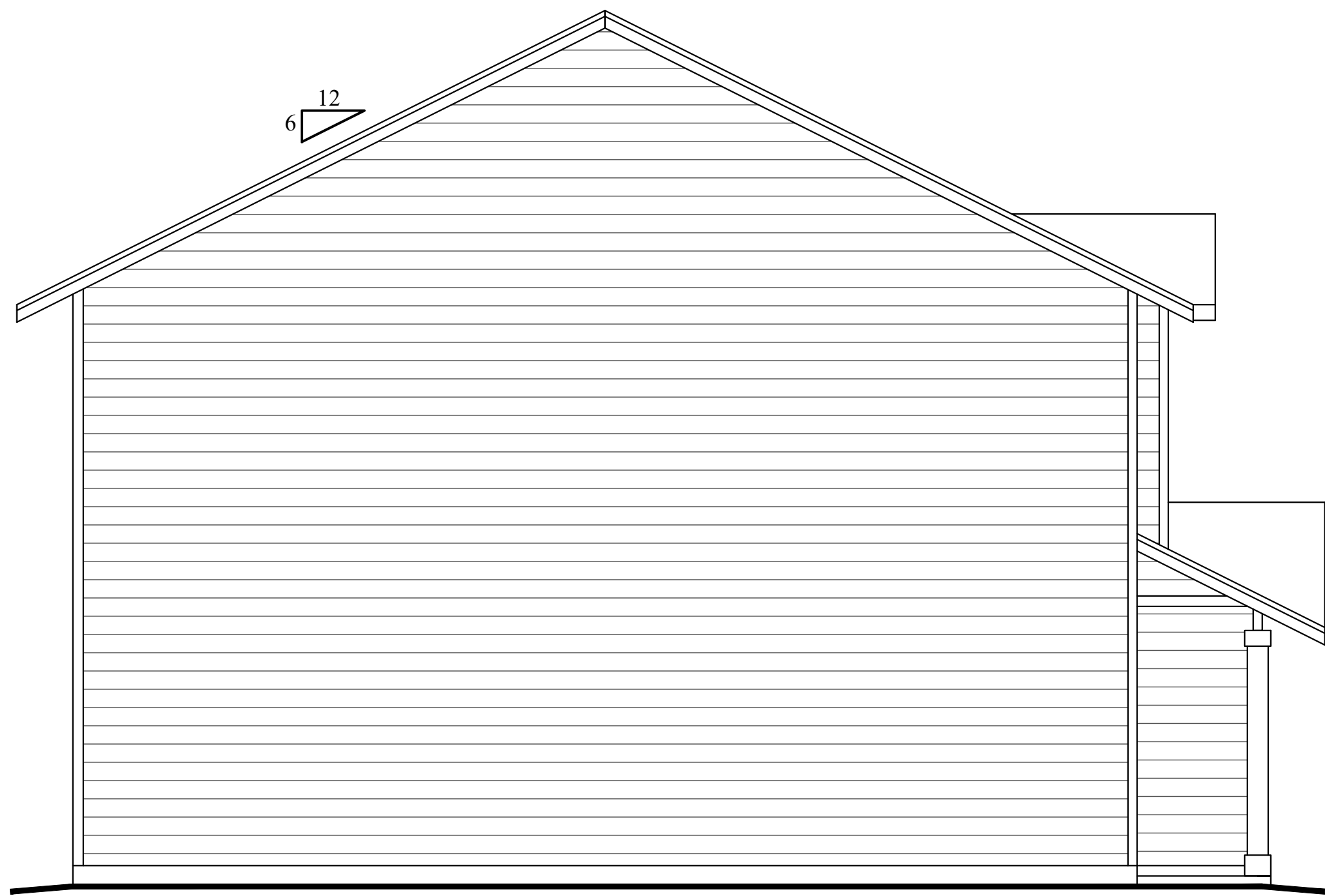
LEFT ELEVATION 1/4" = 1'-0"
