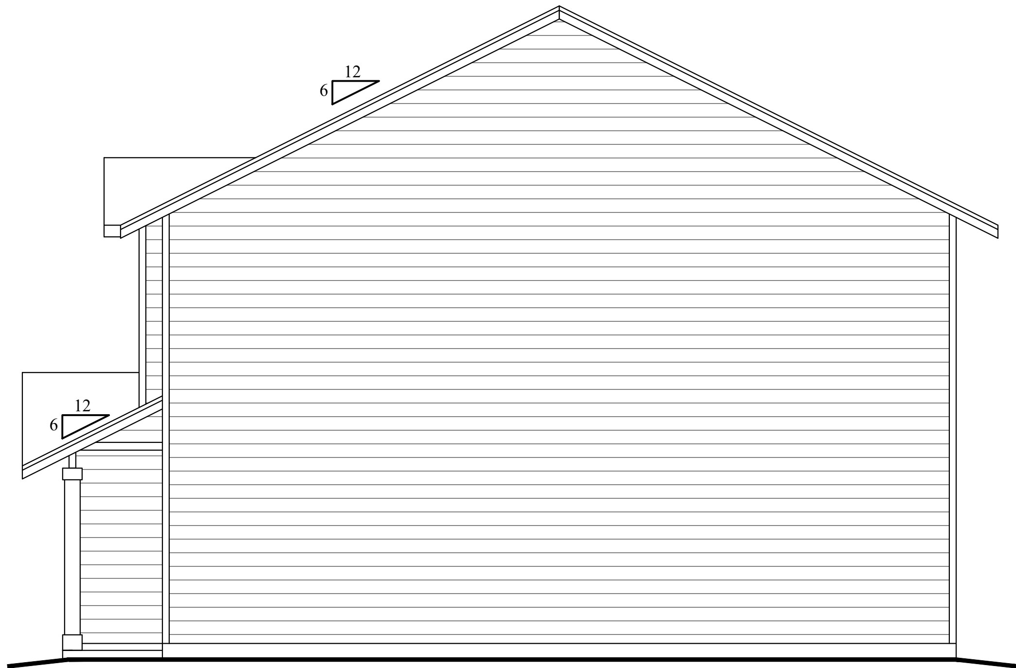
RIGHT ELEVATION 1/4" = 1'-0"
