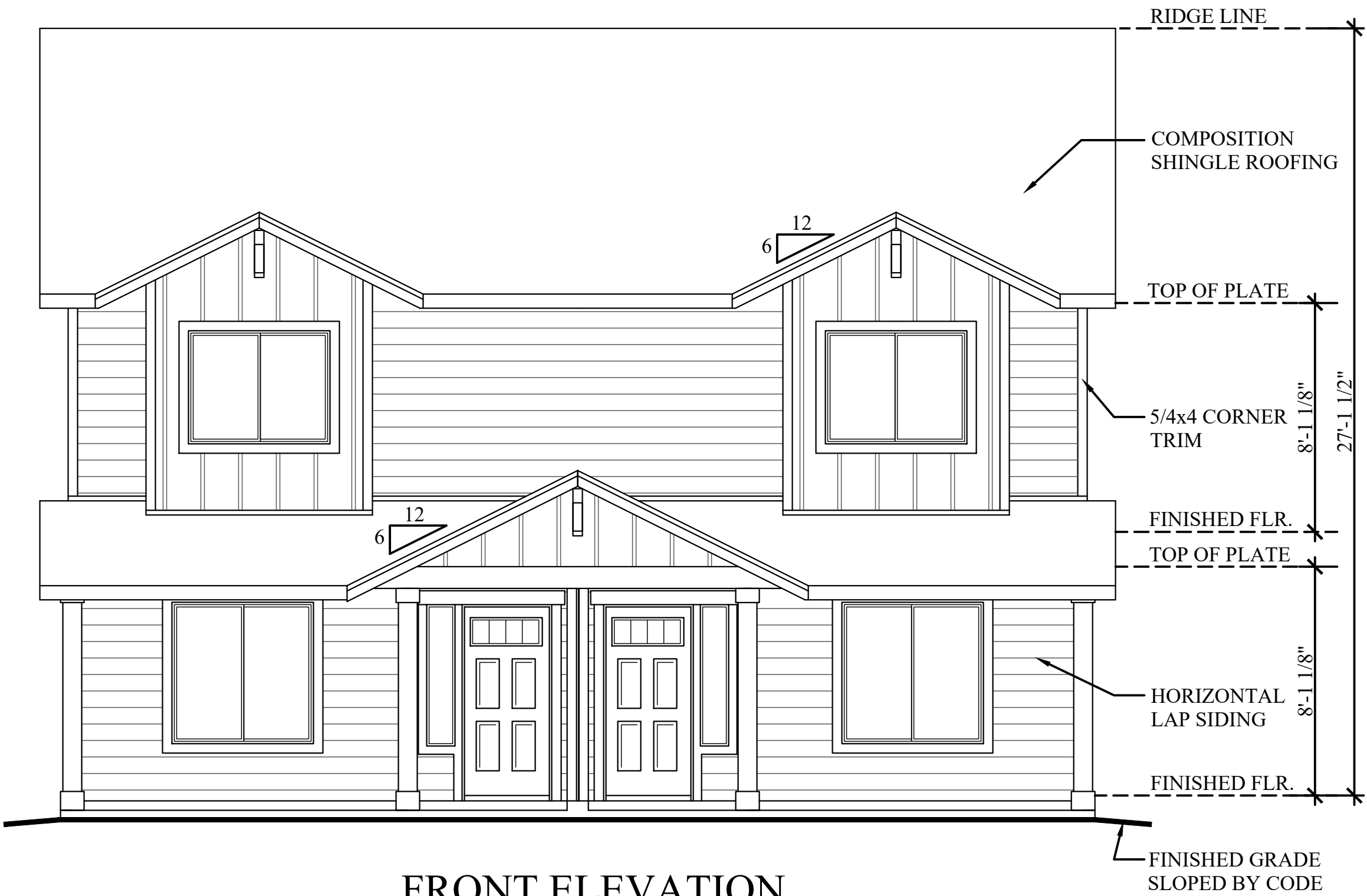
FRONT ELEVATION 1/4" = 1'-0"
