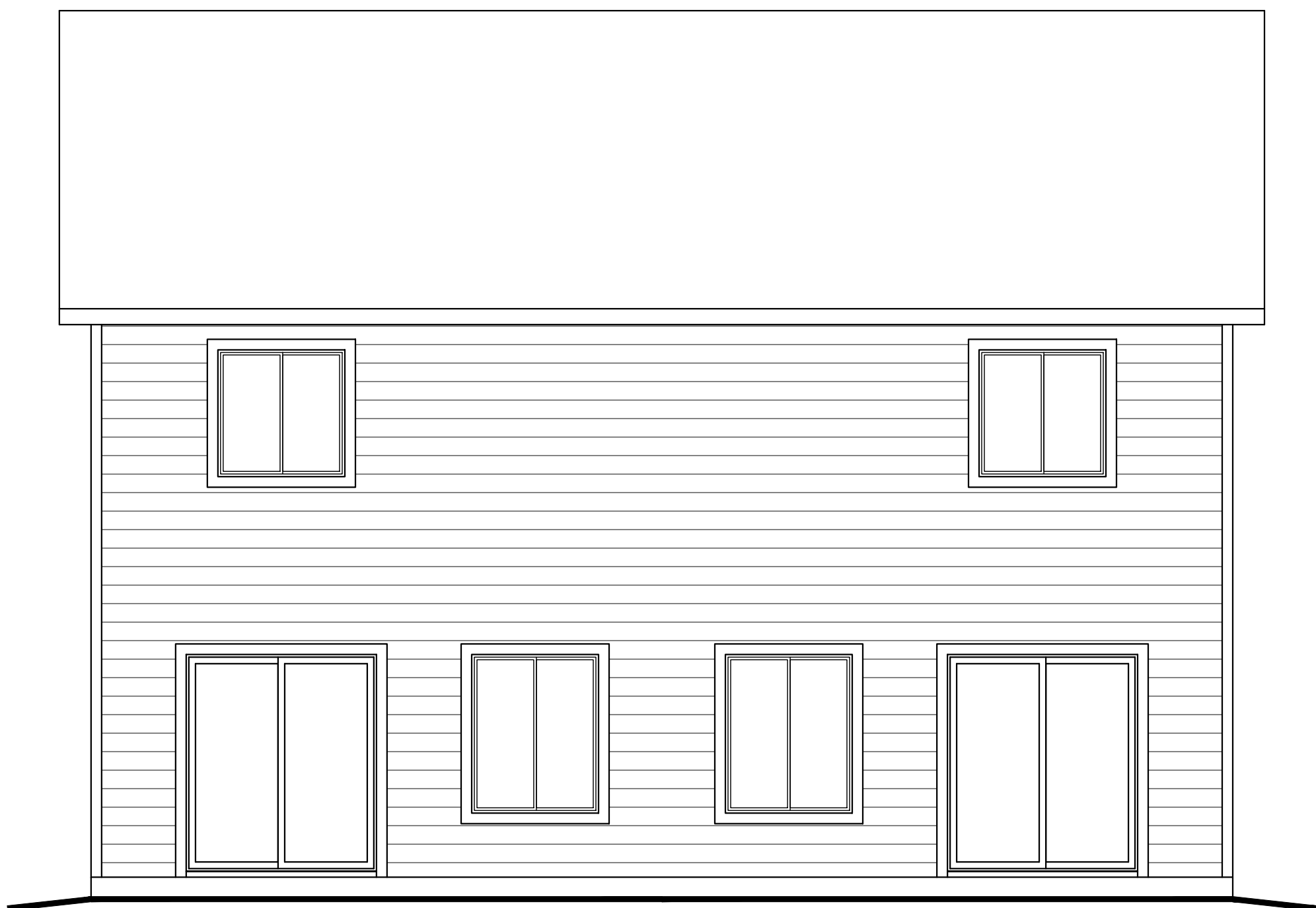
REAR ELEVATION 1/4" = 1'-0"
