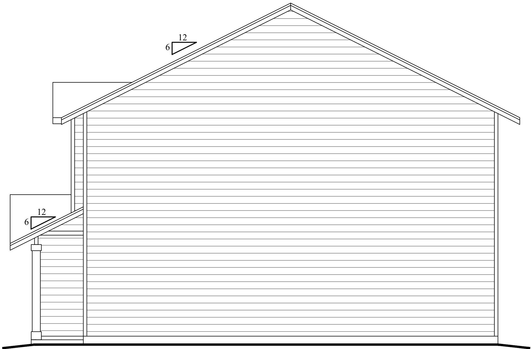
RIGHT ELEVATION 1/4" = 1'-0"
