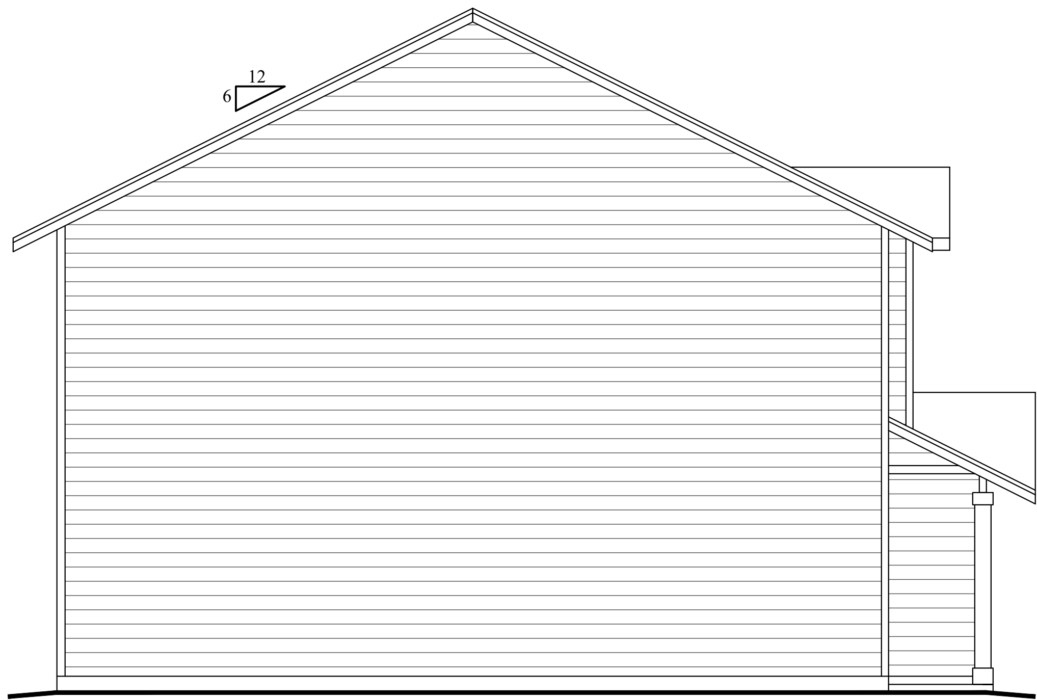
LEFT ELEVATION 1/4" = 1'-0"
