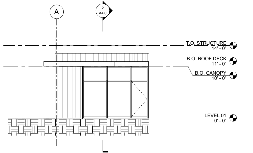
3 ELEVATION - EAST COURTYARD 3/16" = 1'-0"
