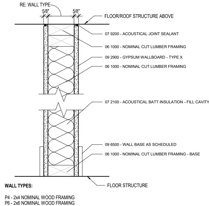
1 P( ) - INTERIOR WOOD FRAMED PARTITION 3" = 1'-0"
