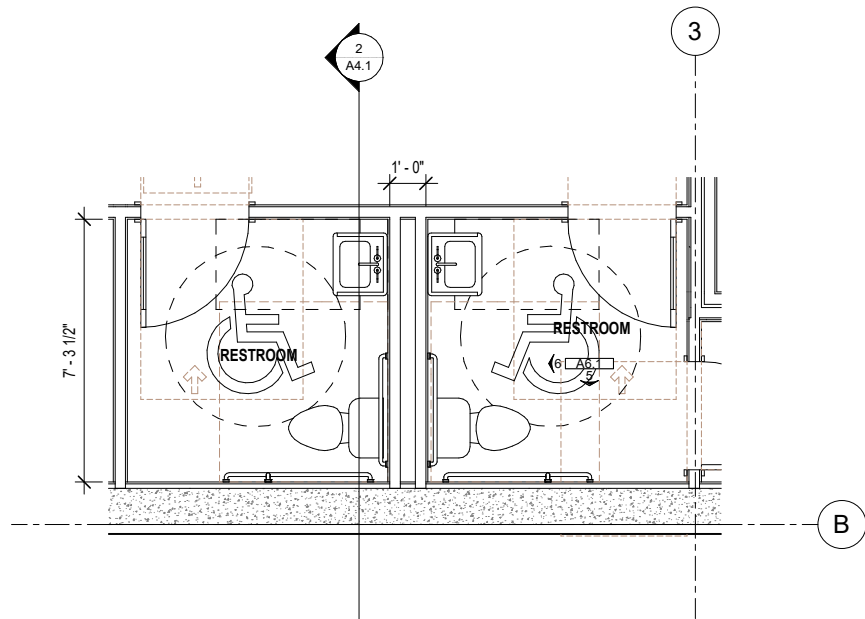
1 ENLARGED PLAN - LEVEL 0 RESTROOMS 3/8" = 1'-0"
