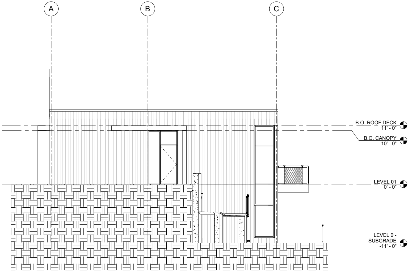
1 ELEVATION EAST 3/16" = 1'-0"
