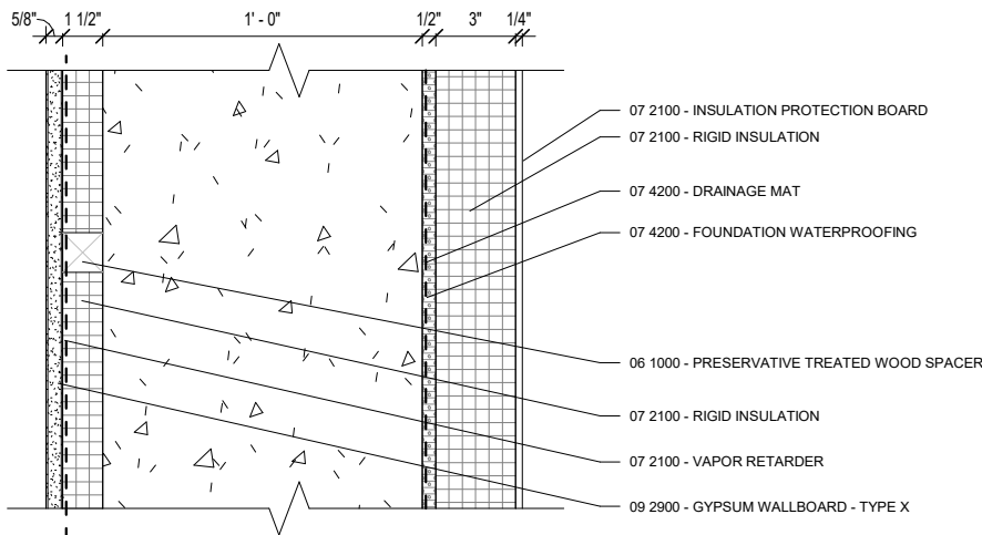
3 FWS_CONC1 - CONCRETE FOUNDATION WALL 3" = 1'-0"
