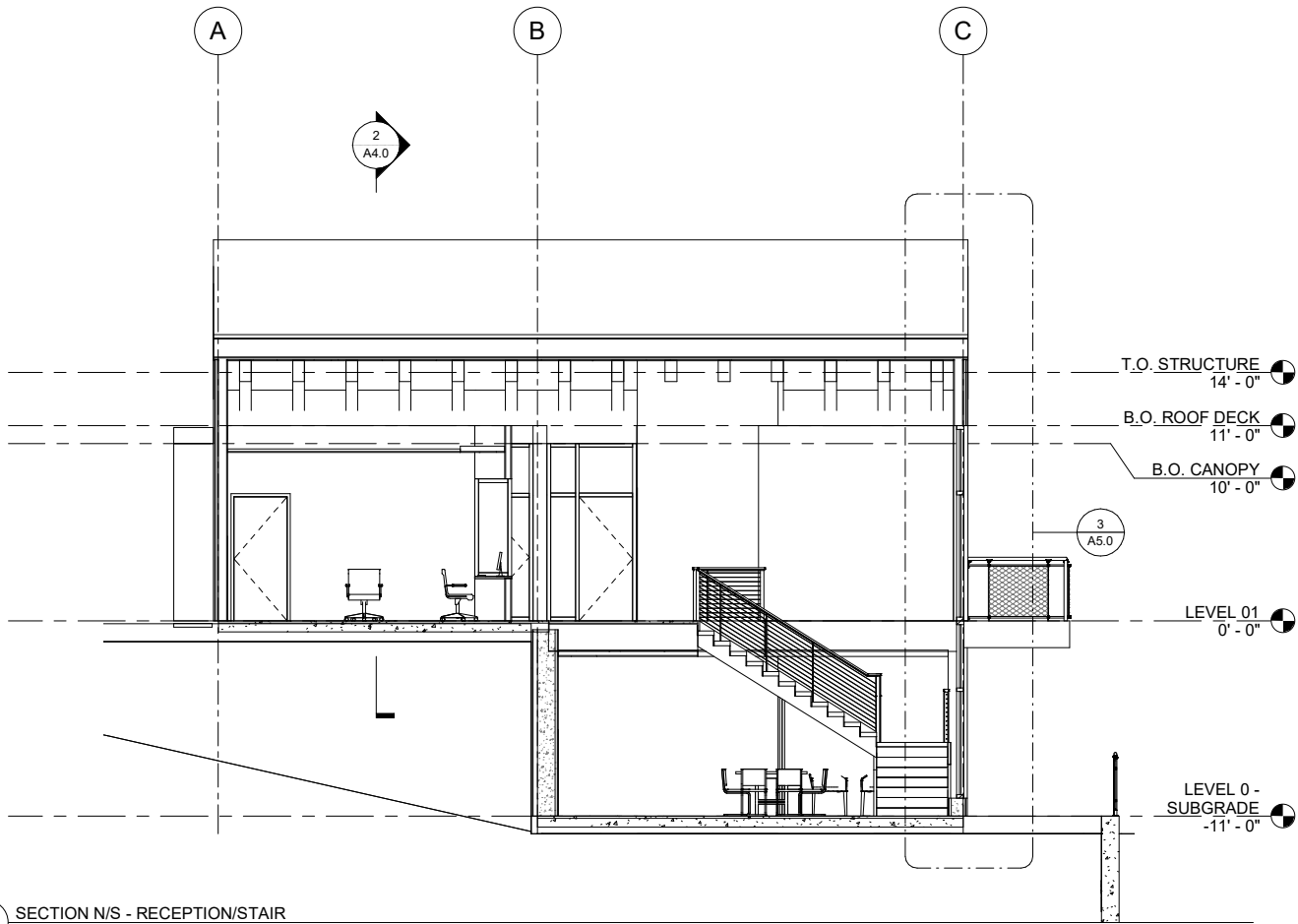
1 SECTION N/S - RECEPTION/STAIR 3/16" = 1'-0"
