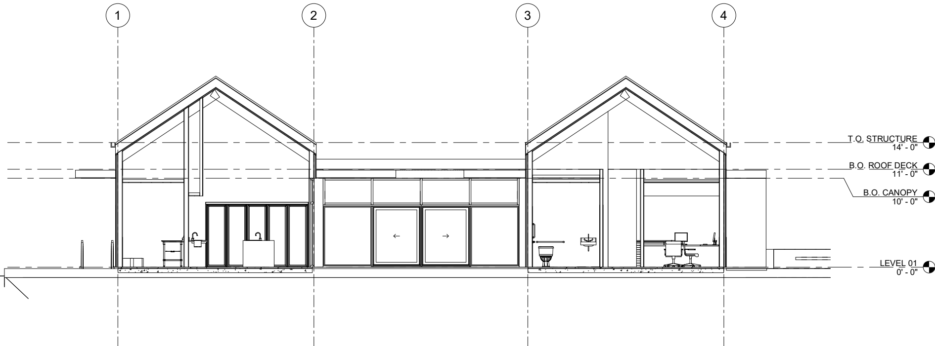
2 SECTION E/W - COURTYARD 3/16" = 1'-0"
