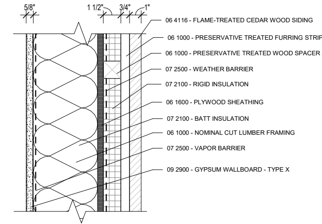
1 WS_WD1 - EXTERIOR WOOD CLAD WALL SYSTEM 3" = 1'-0"
