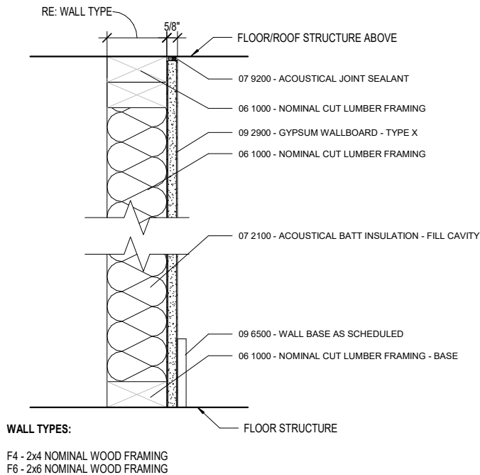
2 F( ) - INTERIOR WOOD FRAMED FURRING WALL 3" = 1'-0"
