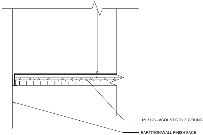
5 CLG-ACT1 - ACOUSTIC TILE CEILING 3" = 1'-0"
