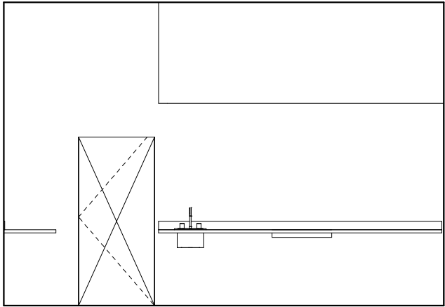
3 KITCHEN WEST 3/8" = 1'-0"
