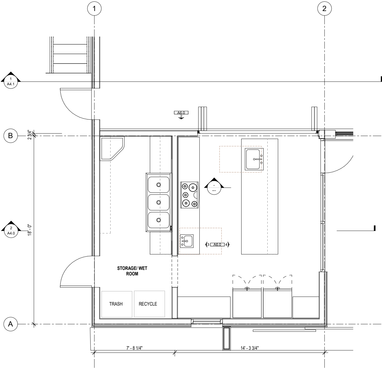
1 ENLARGED PLAN - LEVEL 01 - KITCHEN 3/8" = 1'-0"
