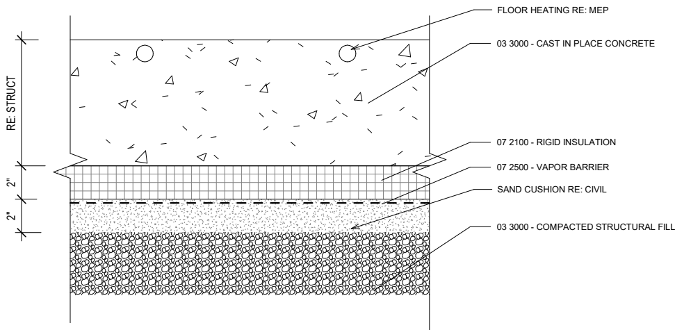
6 FS_CONC2 - SLAB ON GRADE CONCRETE FLOOR SYSTEM 3" = 1'-0"
