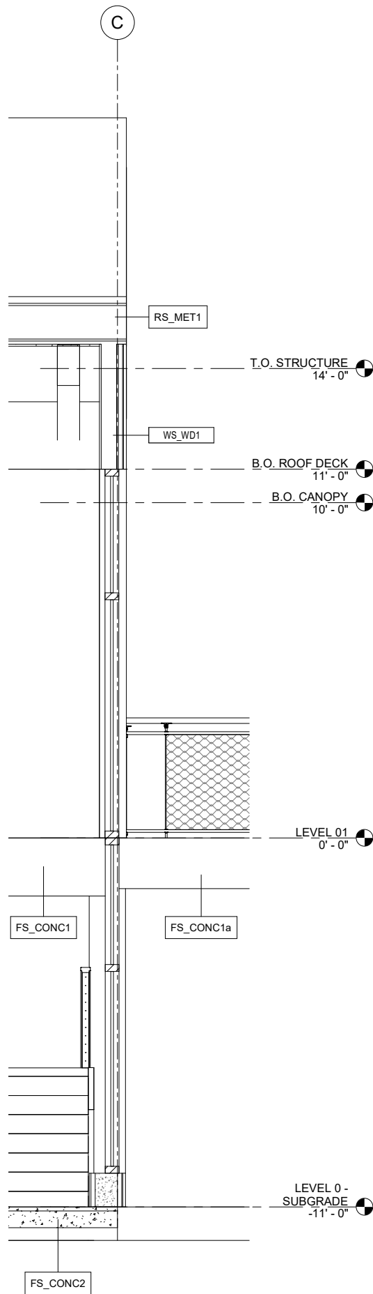
3 WALL SECTION DECK AT DAYLIGHT BASEMENT 1/2" = 1'-0"
