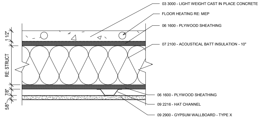
NOTE: FLOOR TYPE FS_CONC1a EXCLUDES BATT INSULATION, FLOOR HEATING, AND GYPSUM WALL BOARD. BOTTOM FACE IS CLAD WITH CEDAR SOFFIT PANELS 6 FS_CONC1 - CONCRETE FLOOR & CEILING SYSTEM 3" = 1'-0"
