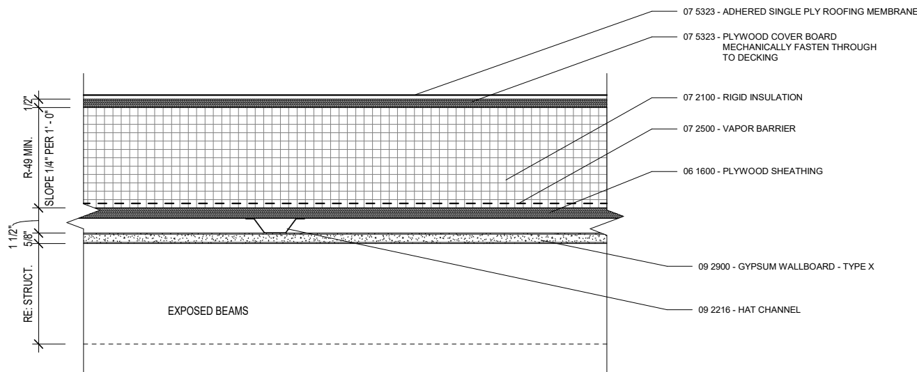
4 RS_EPDM1 - EPDM ROOF SYSTEM 3" = 1'-0"
