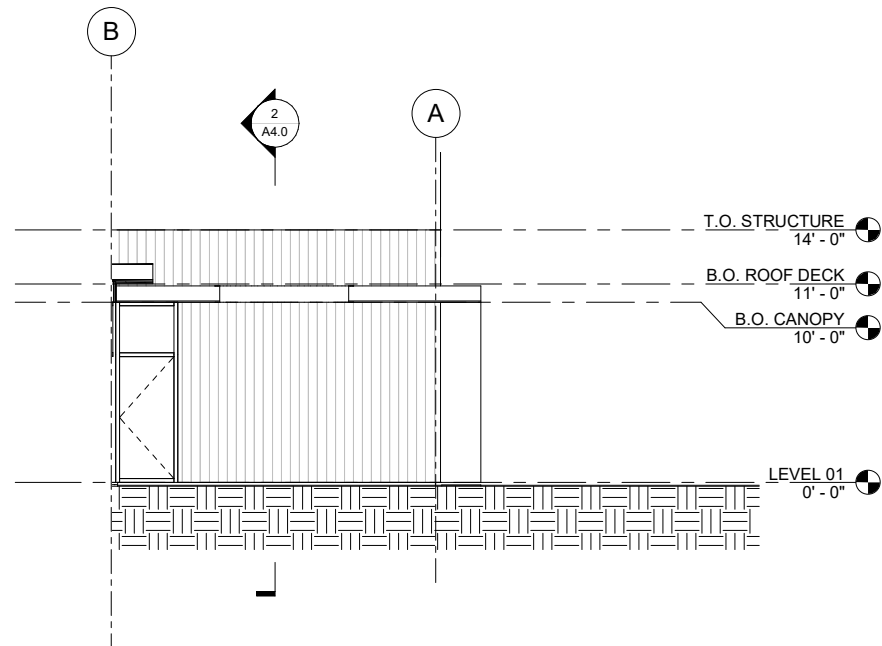
5 ELEVATION - WEST COURTYARD 3/16" = 1'-0"
