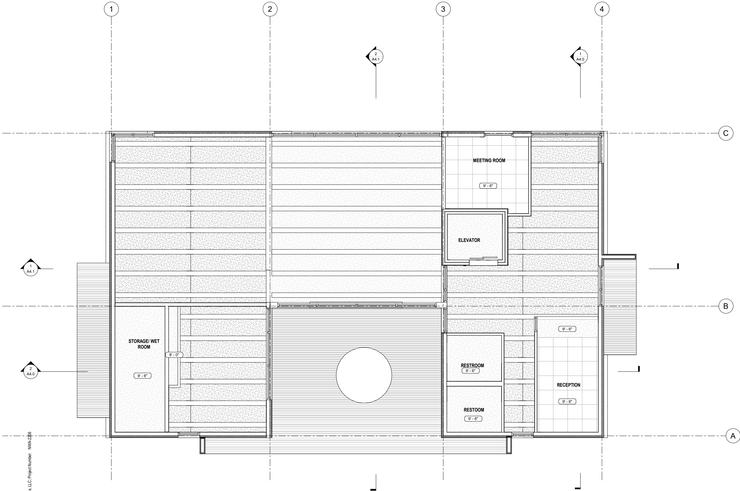
1 REFLECTED CEILING PLAN - LEVEL 01 1/4" = 1'-0"
