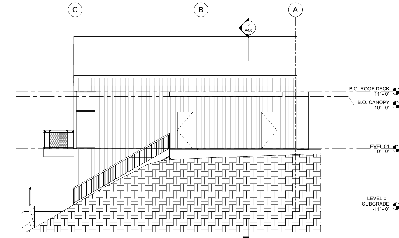
2 ELEVATION WEST 3/16" = 1'-0"
