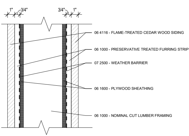
5 WS_WD2 - EXTERIOR WOOD CLAD FIN WALL SYSTEM 3" = 1'-0"
