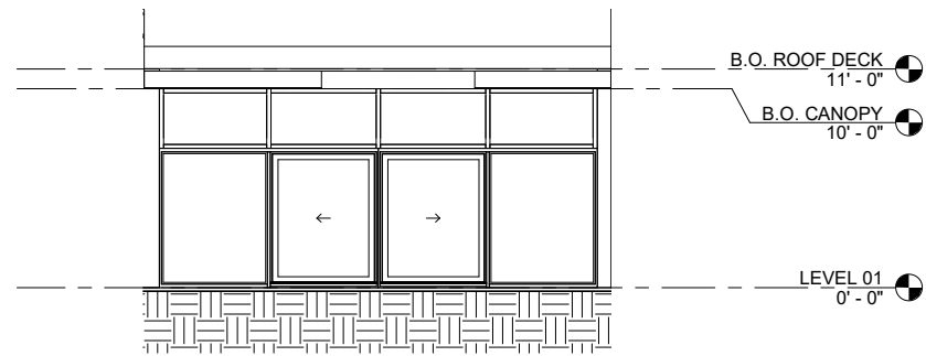
4 ELEVATION - SOUTH COURTYARD 3/16" = 1'-0"
