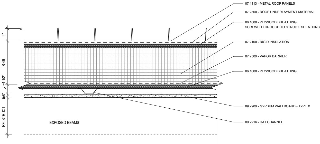
2 RS_MET1 - METAL PANEL ROOF SYSTEM 3" = 1'-0"
