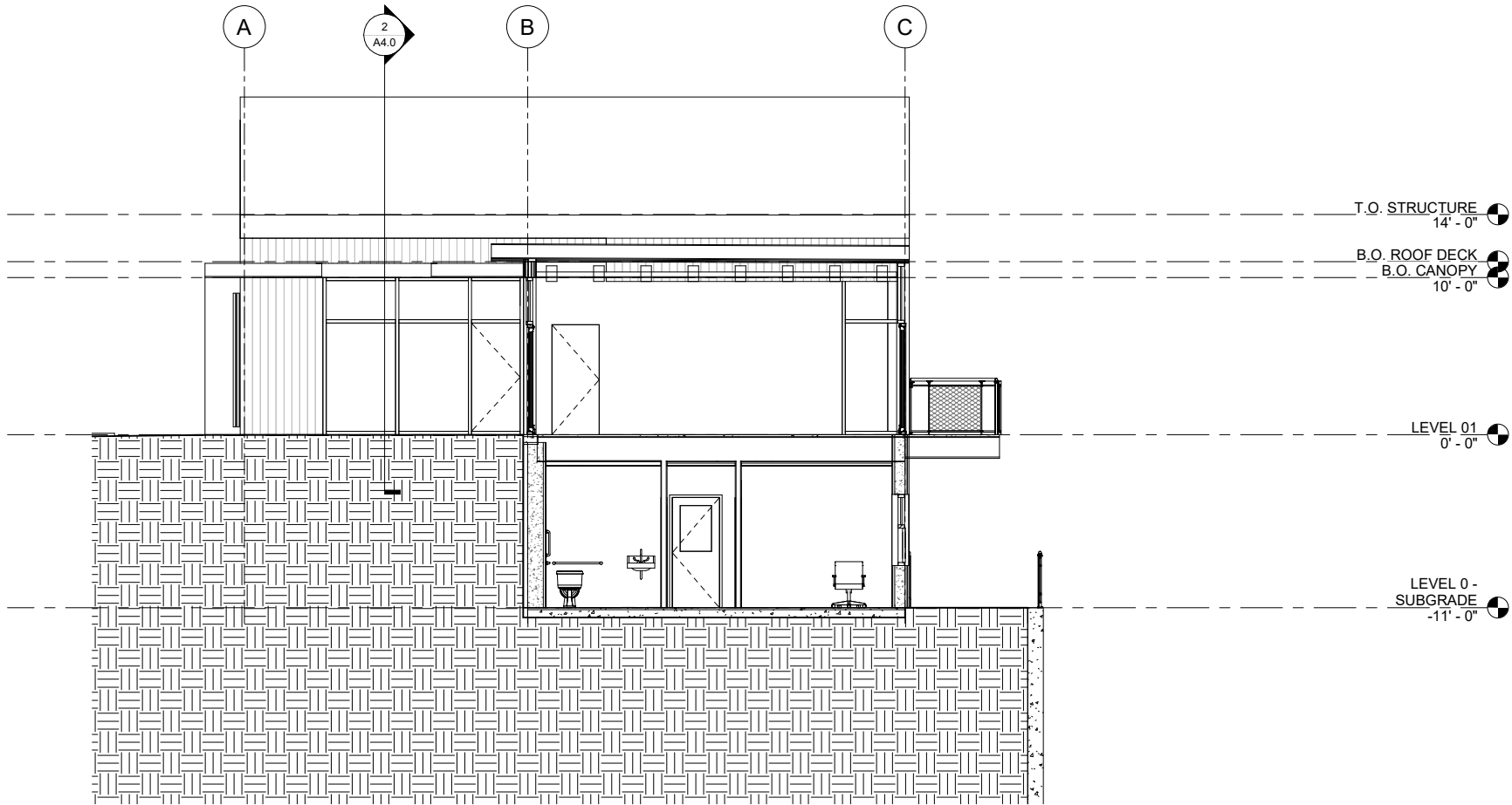
2 SECTION N/S - COURTYARD 3/16" = 1'-0"
