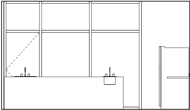
4 KITCHEN EAST 3/8" = 1'-0"
