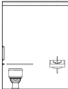
3 LEVEL 1 RESTROOM NORTH 3/8" = 1'-0"
