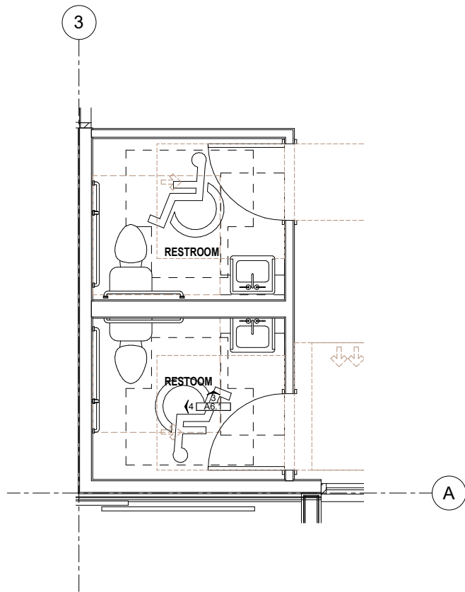
2 ENLARGED PLAN - LEVEL 1 - RESTROOMS 3/8" = 1'-0"
