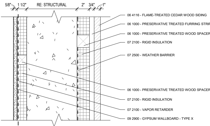
7 WS_CONC1 - CONCRETE FOUNDATION WALL 3" = 1'-0"
