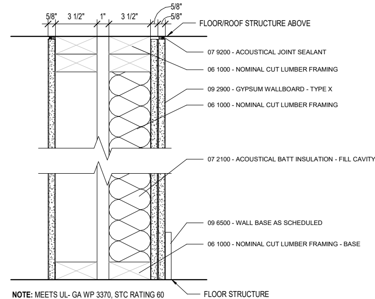
3 SW1 - INTERIOR WOOD FRAMED ELEVATOR SHAFT WALL PARTITION 3" = 1'-0"
