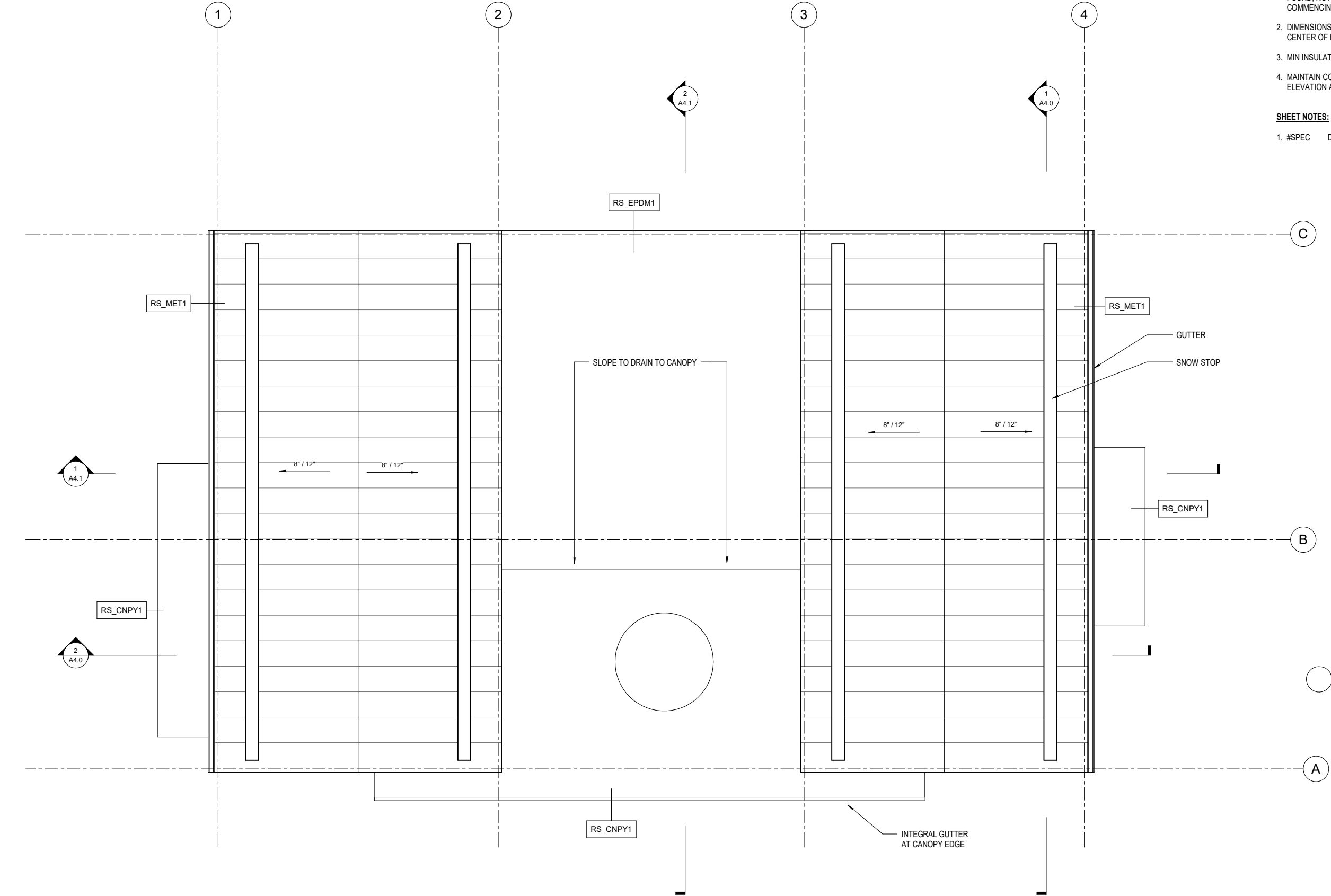
1 ROOF PLAN 1/4" = 1'-0"
