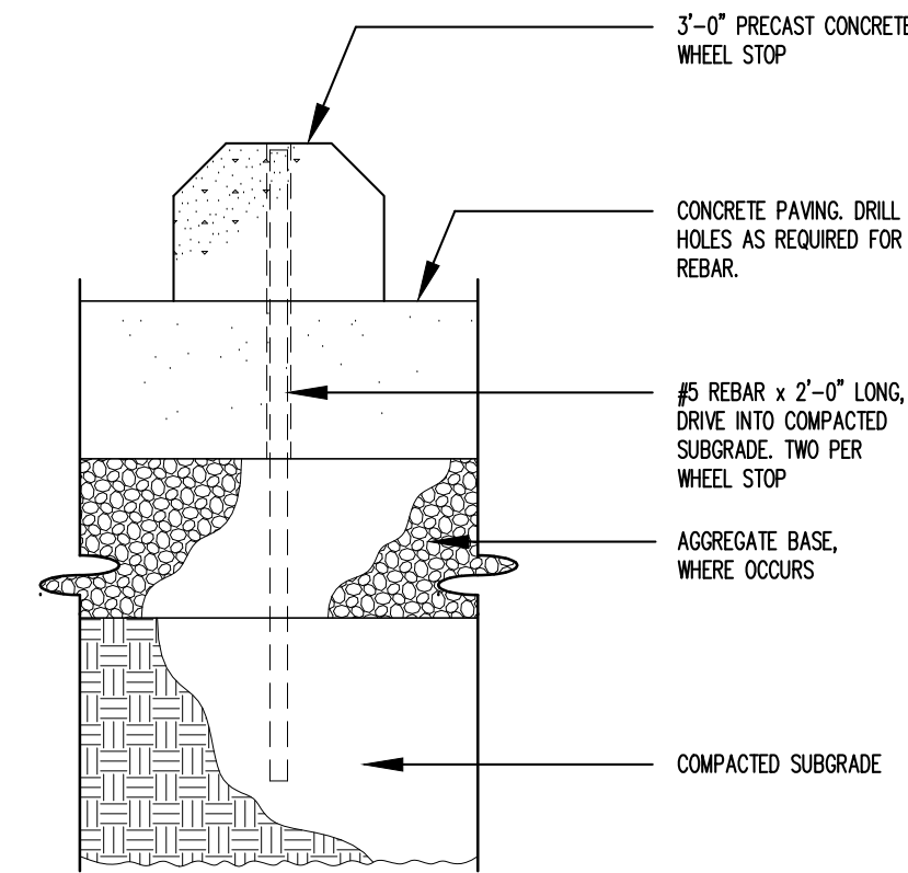
05 CONCRETE WHEEL STOP SCALE: 1-1/2" = 1'-0"
