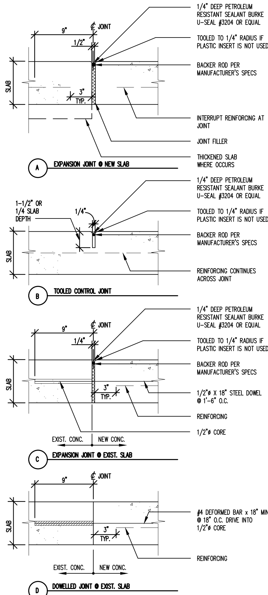
03 CONCRETE JOINTS SCALE: 1-1/2" = 1'-0"
