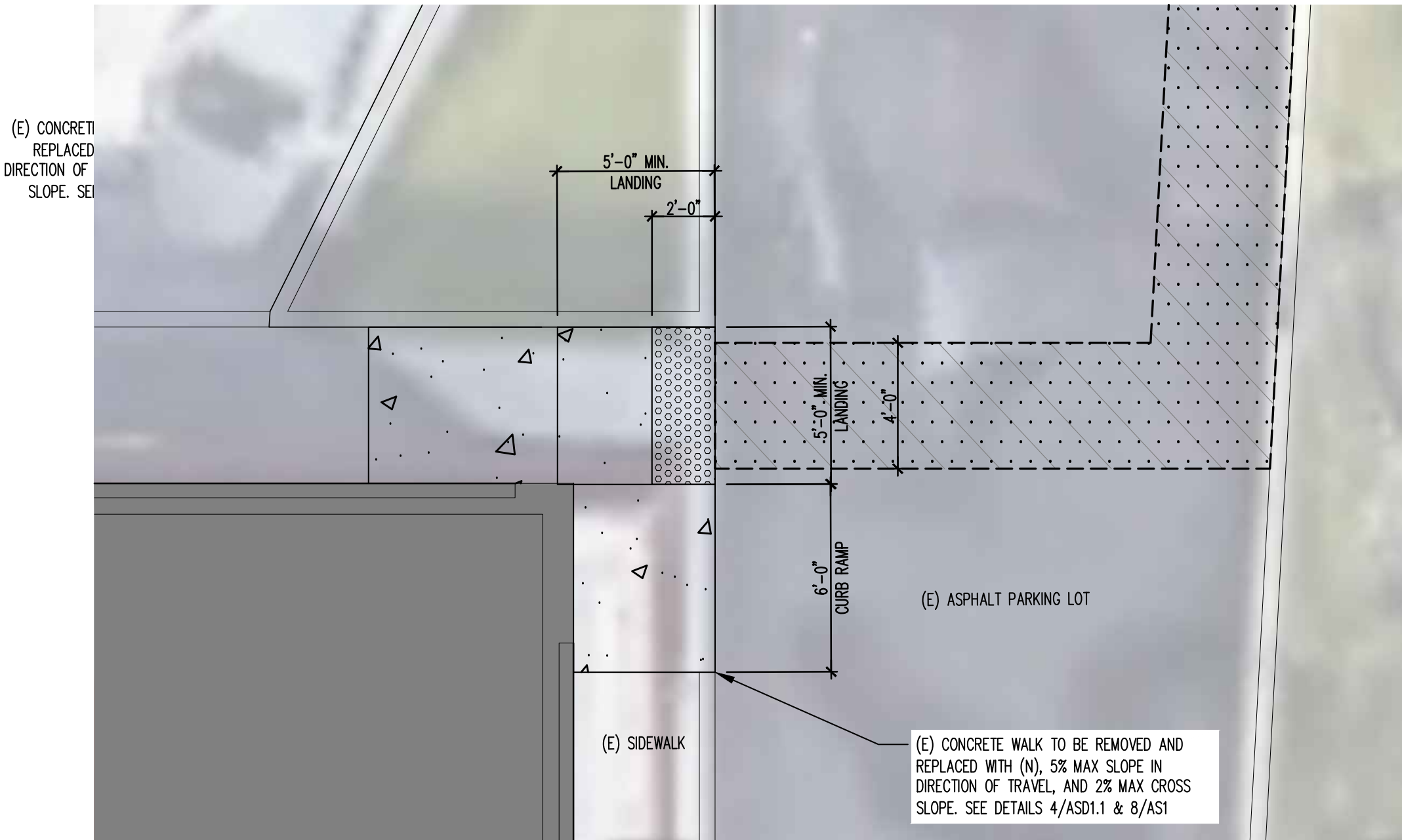
07 ENLARGED SITE PLAN SCALE: 1/4" = 1'-0"
