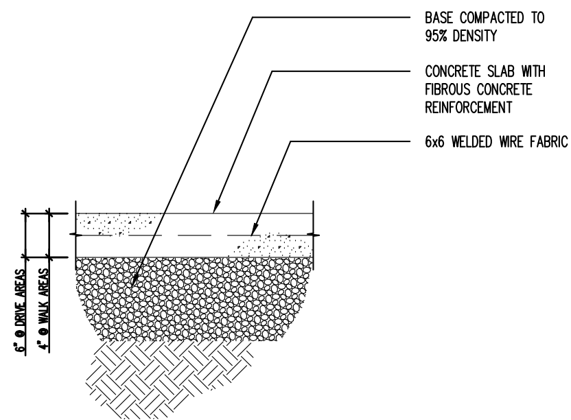
02 CONC. SIDEWALK/PAVING SECT. (TYP) SCALE: 1" = 1'-0"
