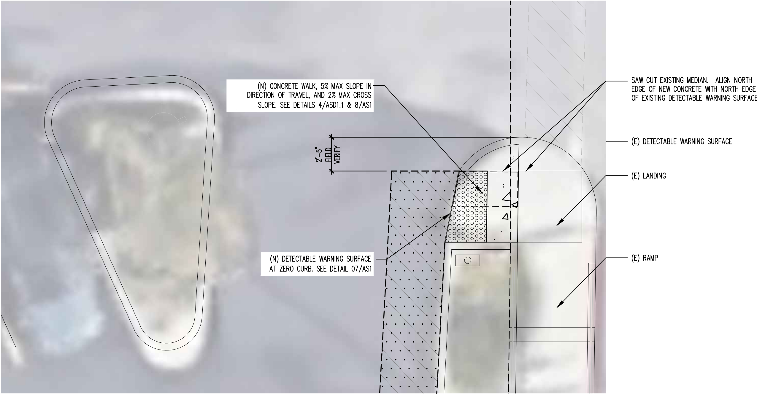
06 ENLARGED SITE PLAN SCALE: 1/4" = 1'-0"
