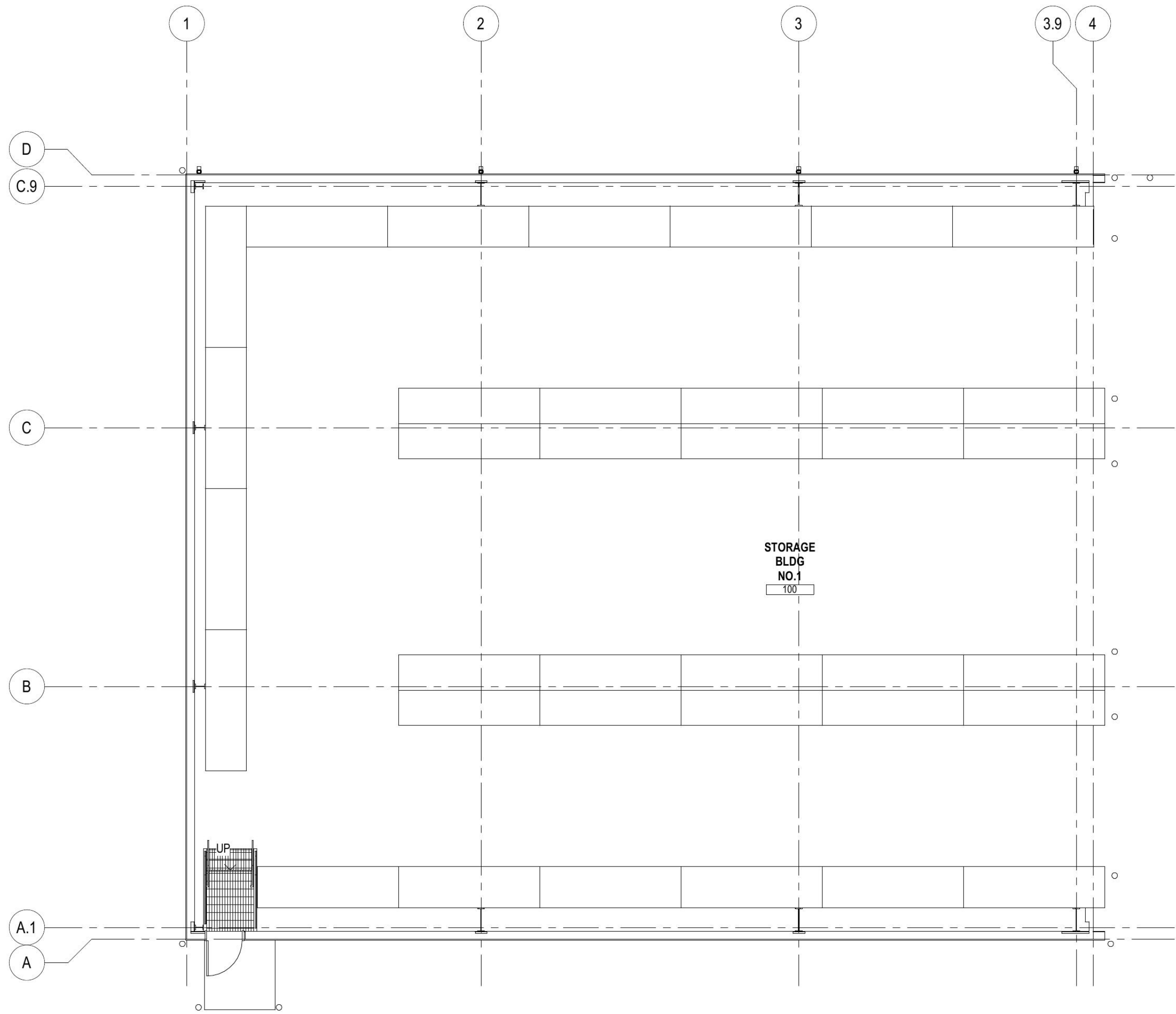
1 LIFE SAFETY PLAN 1/8" = 1'-0"
