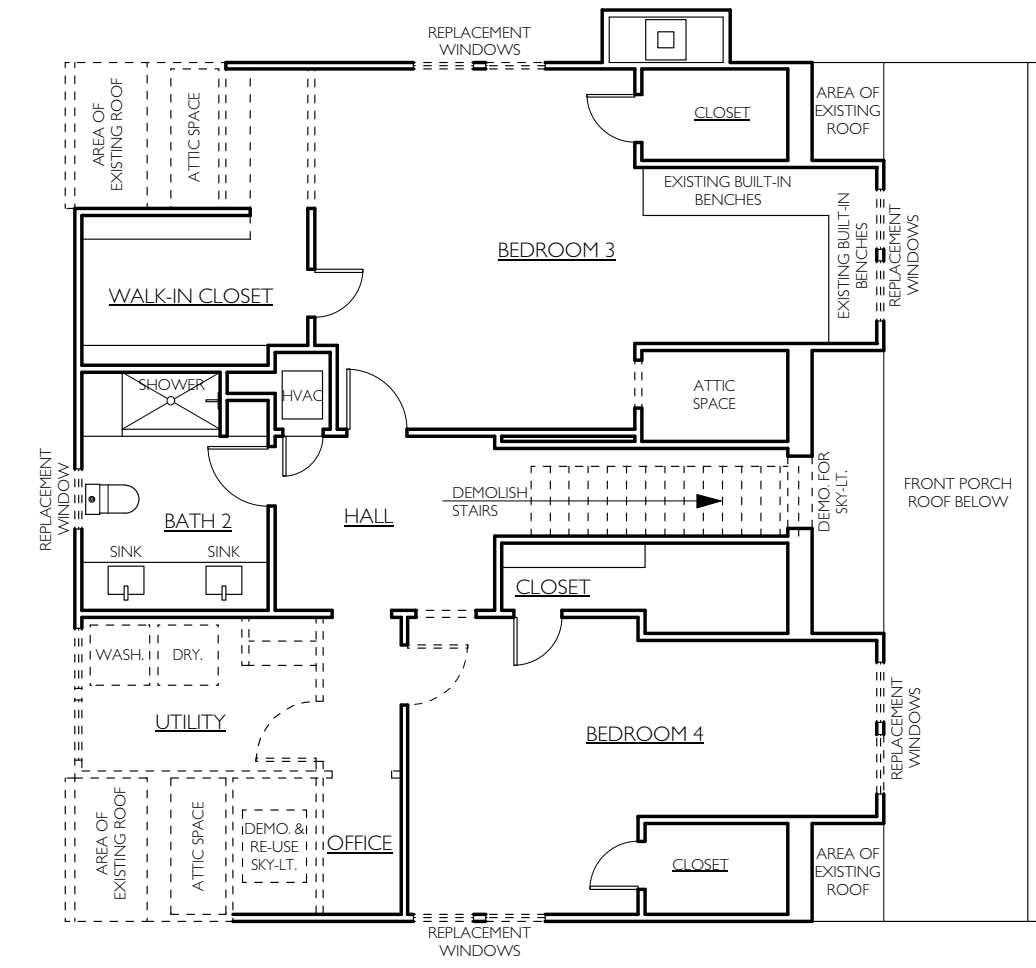
3 SECOND FLOOR DEMOLITION PLAN SCALE: 1/8" = 1'-0"
