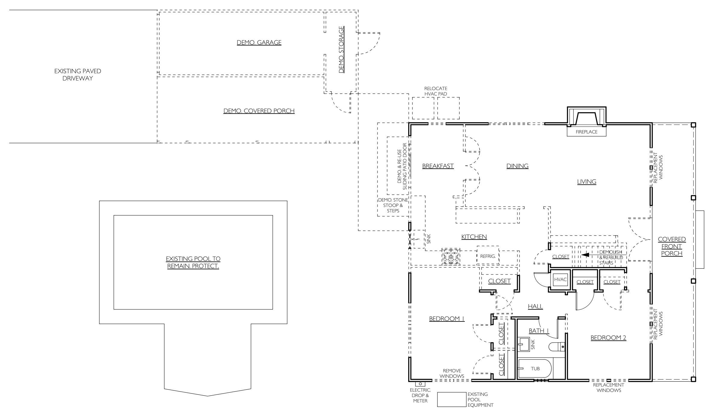
2 FIRST FLOOR DEMOLITION PLAN SCALE: 1/8" = 1'-0"
